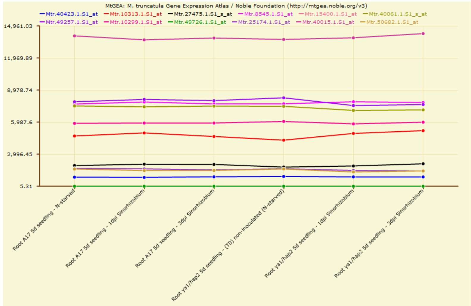
Figure S3 Expression data of Mt14-3-3 genes after an S. meliloti infection from the Medicago gene atlas ( http://mtgea.noble.org/v3/ ). The expression levels of the Mt14-3-3 genes in roots were analyzed at different time points (1 and 3 dpi) after S. meliloti infection.
