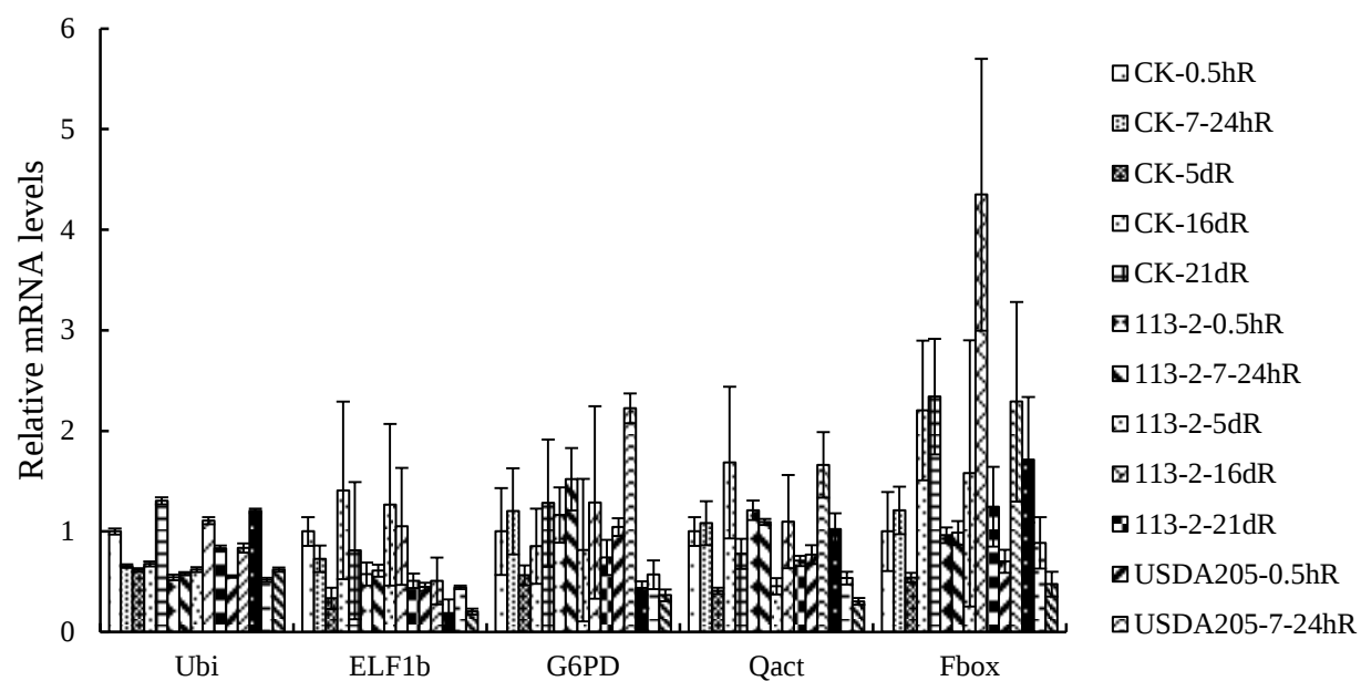
Supplemental Figure S3 The stability assay of five references genes in 15 soybean roots samples.
