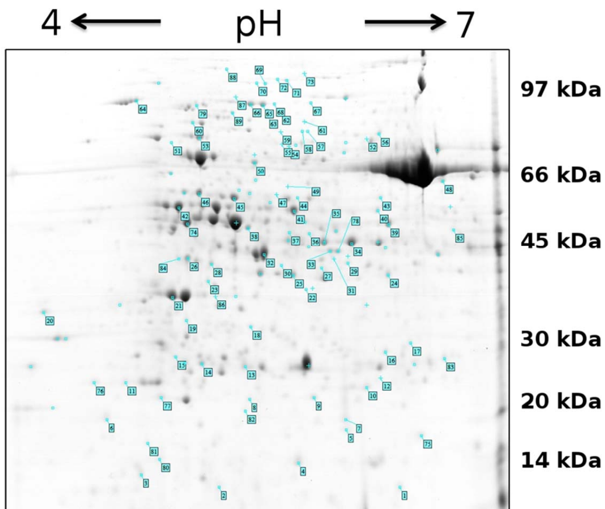
Supplementary Image S3. Representative two-dimensional electrophoretic gel obtained during analysis of protein extracts extracted from Maresi leaves. Protein spot labels according to Supplementary Table S4.
