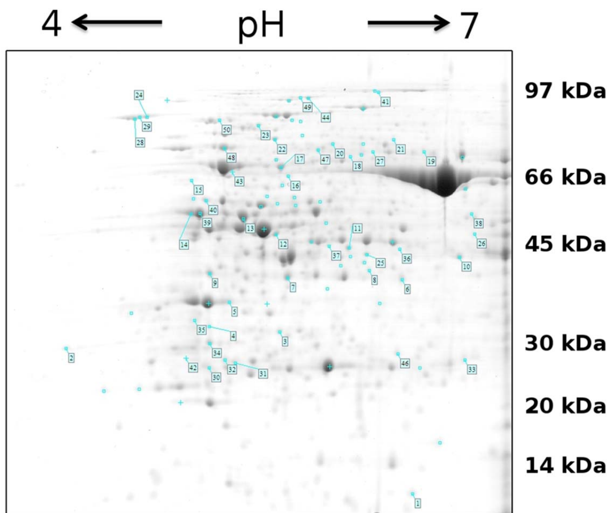
Supplementary Image S4. Representative two-dimensional electrophoretic gel obtained during analysis of protein extracts extracted from Cam/B1/CI leaves. Protein spot labels according to Supplementary Table S5.
