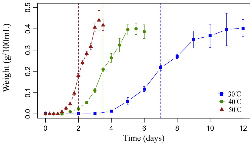
Growth on R 2 A-glucose media
