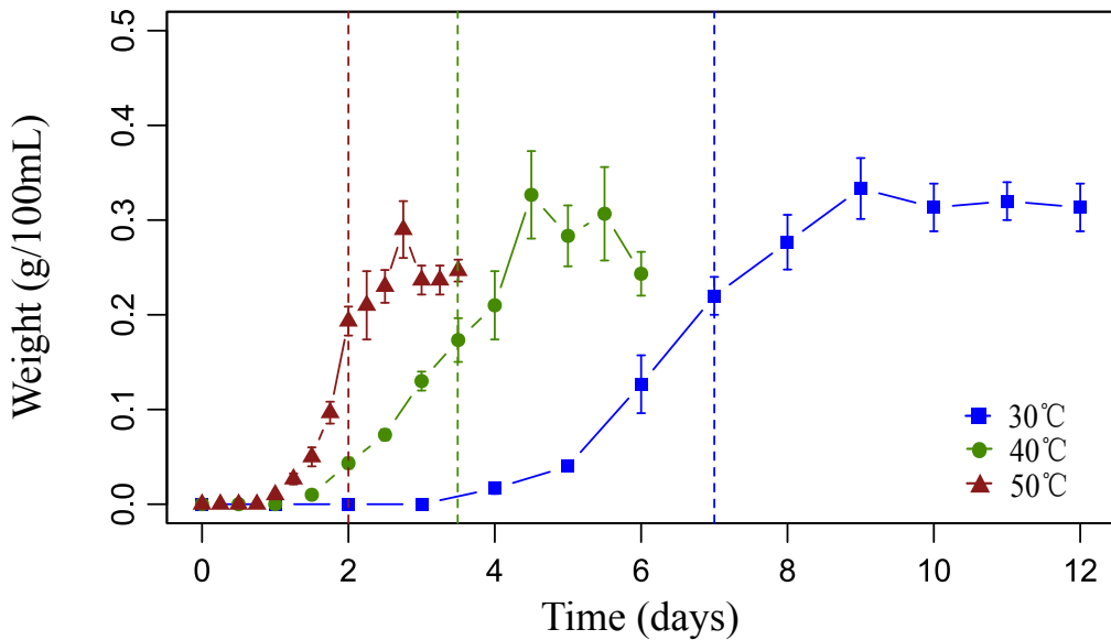
Growth on R 2 A-CMC media
