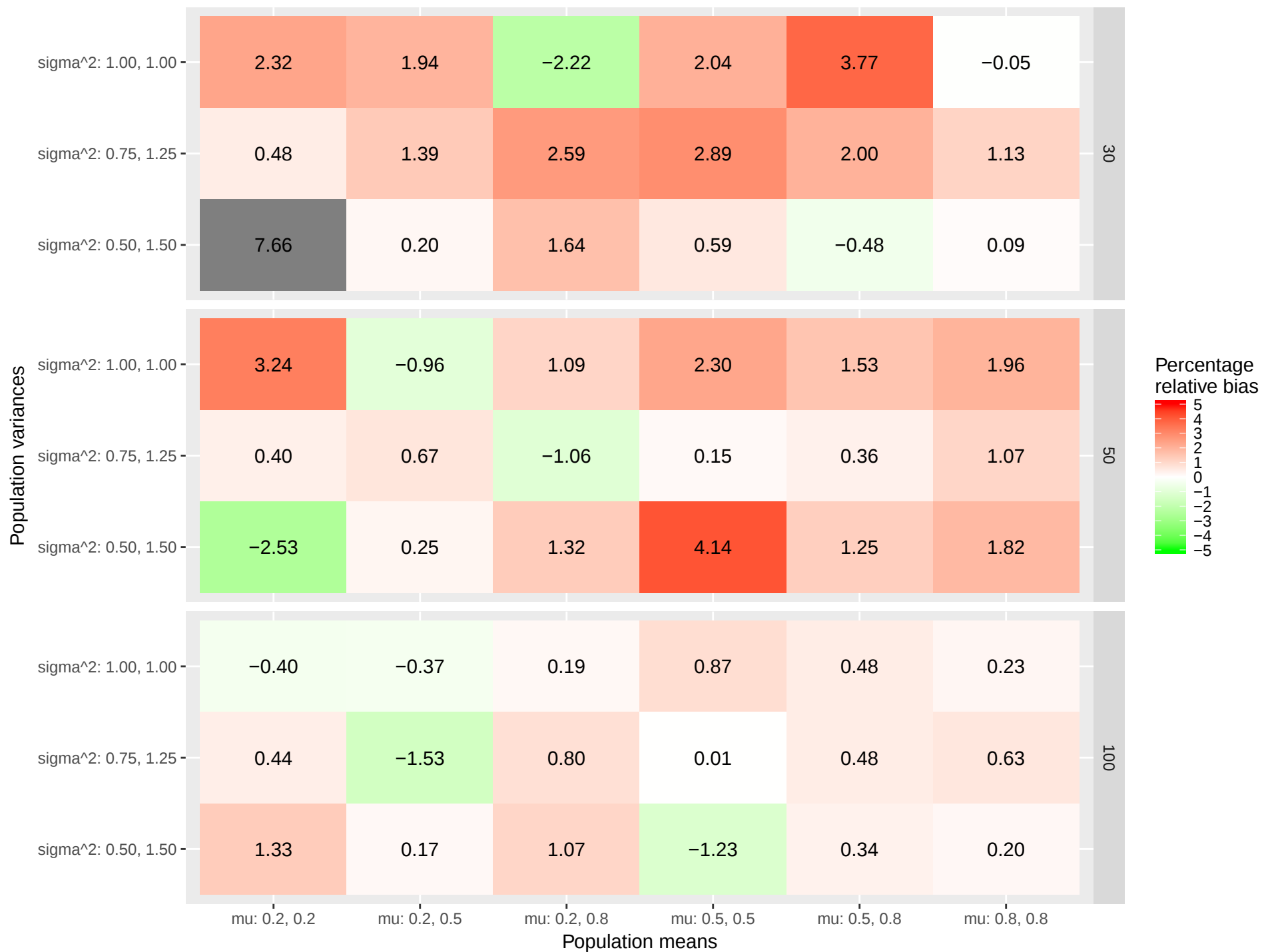
Relative Percentage Bias of the Second Parameter Estimates without the Assumption of Homogeneity of Variances for Multiple Treatment Studies
