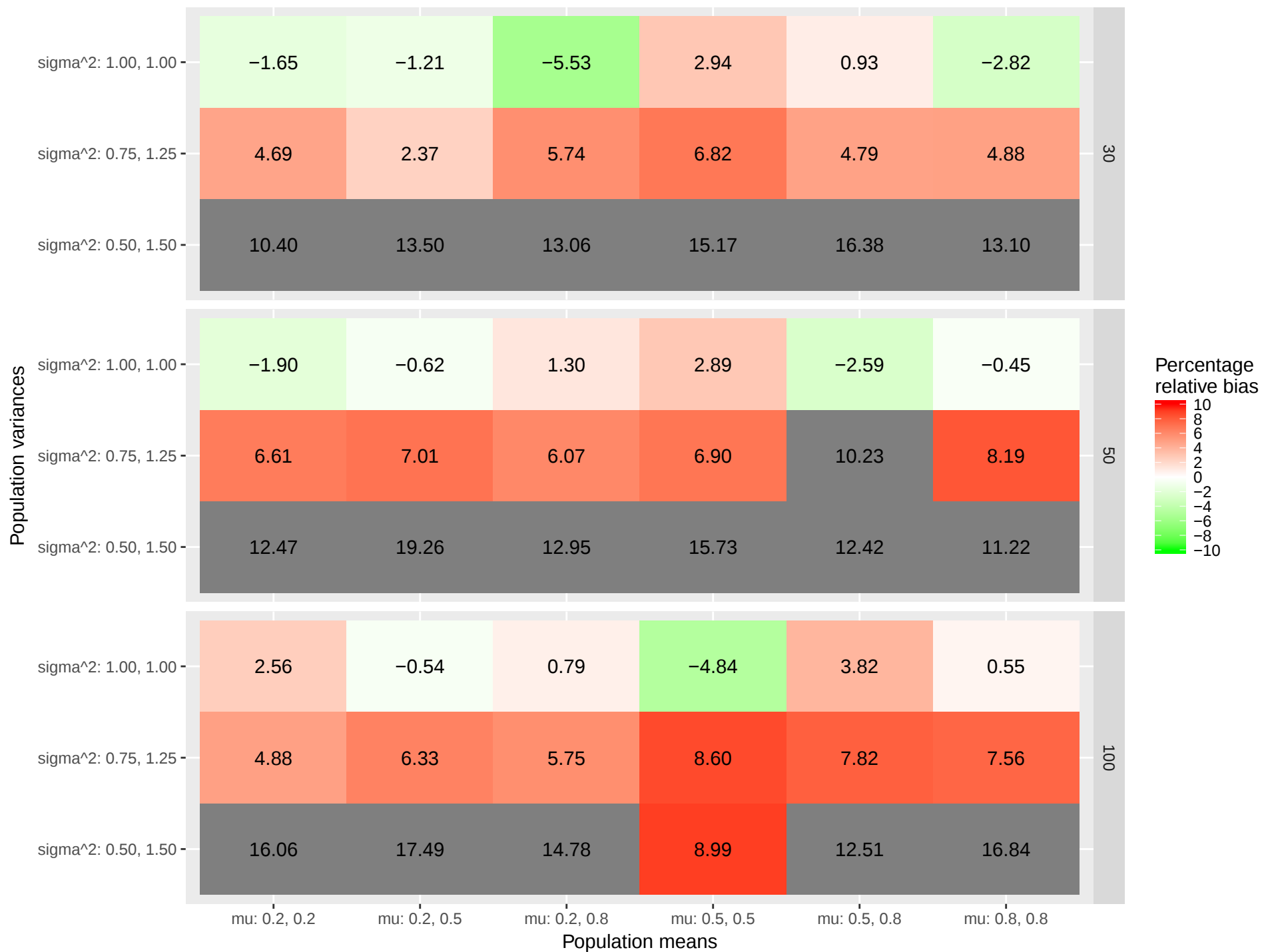
Relative Percentage Bias of the First Estimated Standard Errors with the Assumption of Homogeneity of Variances for Multiple Treatment Studies
