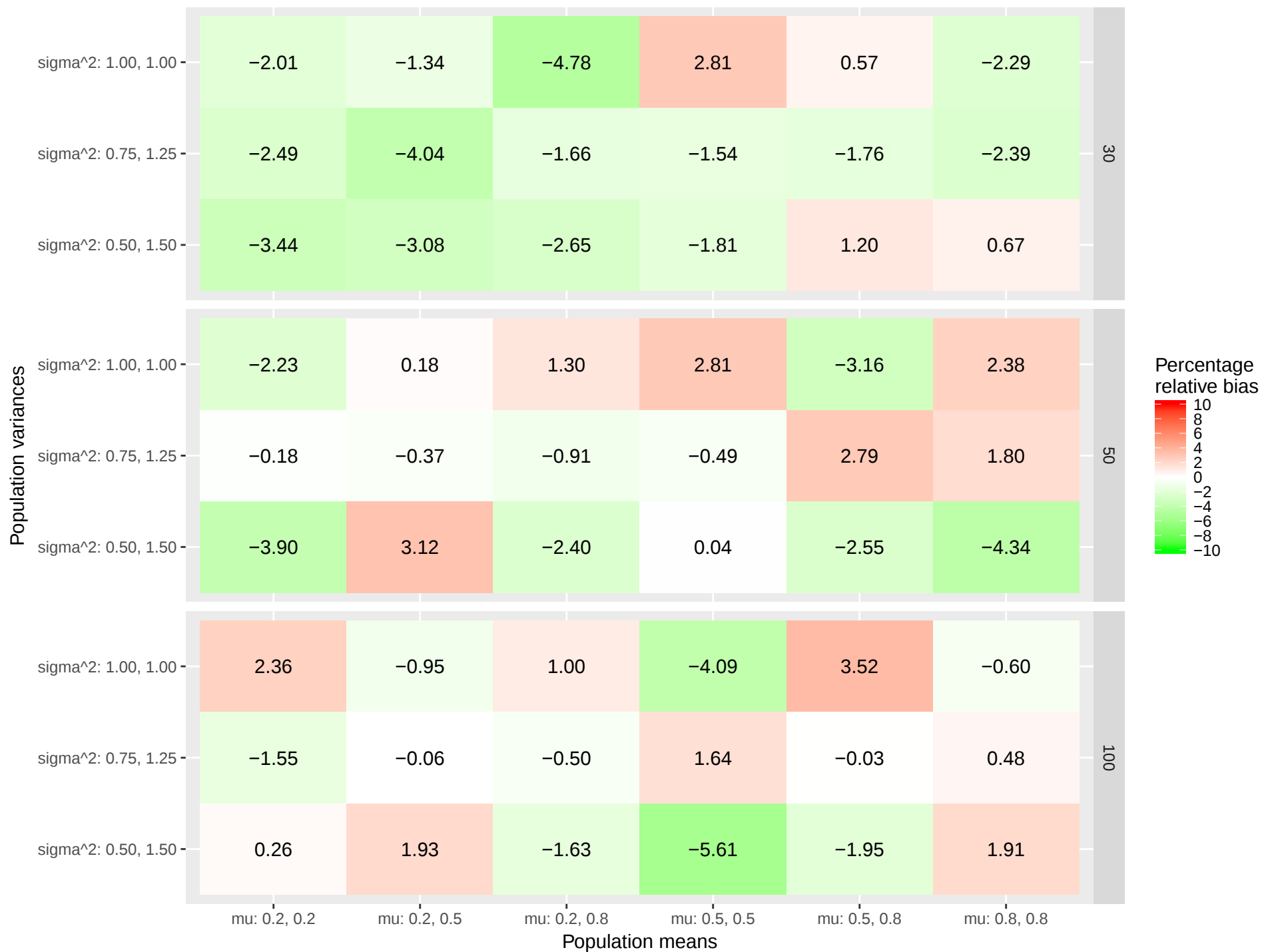
Relative Percentage Bias of the First Estimated Standard Errors without the Assumption of Homogeneity of Variances for Multiple Treatment Studies
