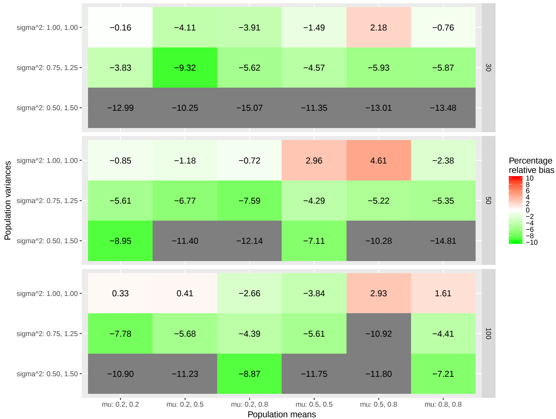
Relative Percentage Bias of the Second Estimated Standard Errors with the Assumption of Homogeneity of Variances for Multiple Treatment Studies
