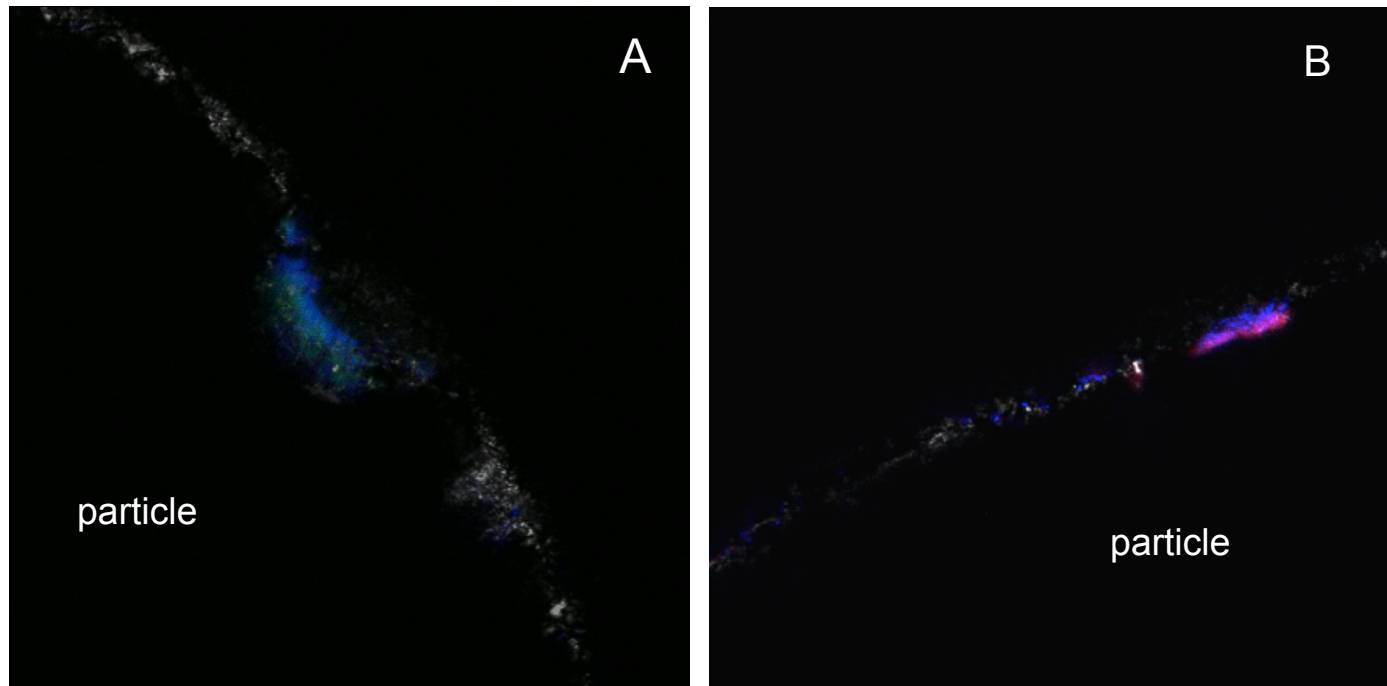
Supplementary Figure 10: Images of sections taken with a confocal microscope of the activated carbon particles used for FISH assays and that show the microbial stratification developed on them. The blue signal corresponds to the DAPI stain while the white signal corresponds to the surface of the particle. For A) signal corresponds to Geobacter cluster and for B) the red signal corresponds to Eubacteria.
