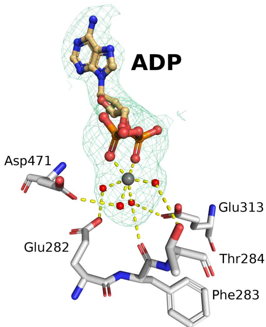
Supplementary Figure S5. Polder omit map for Mg-ADP. Mg^{2+} is showed as gray sphere, water as red spheres and residues that interact with water molecules are labeled. mFo-DFc omit map is contoured at 3 sigma for ADP, Mg^{2+} and waters.
