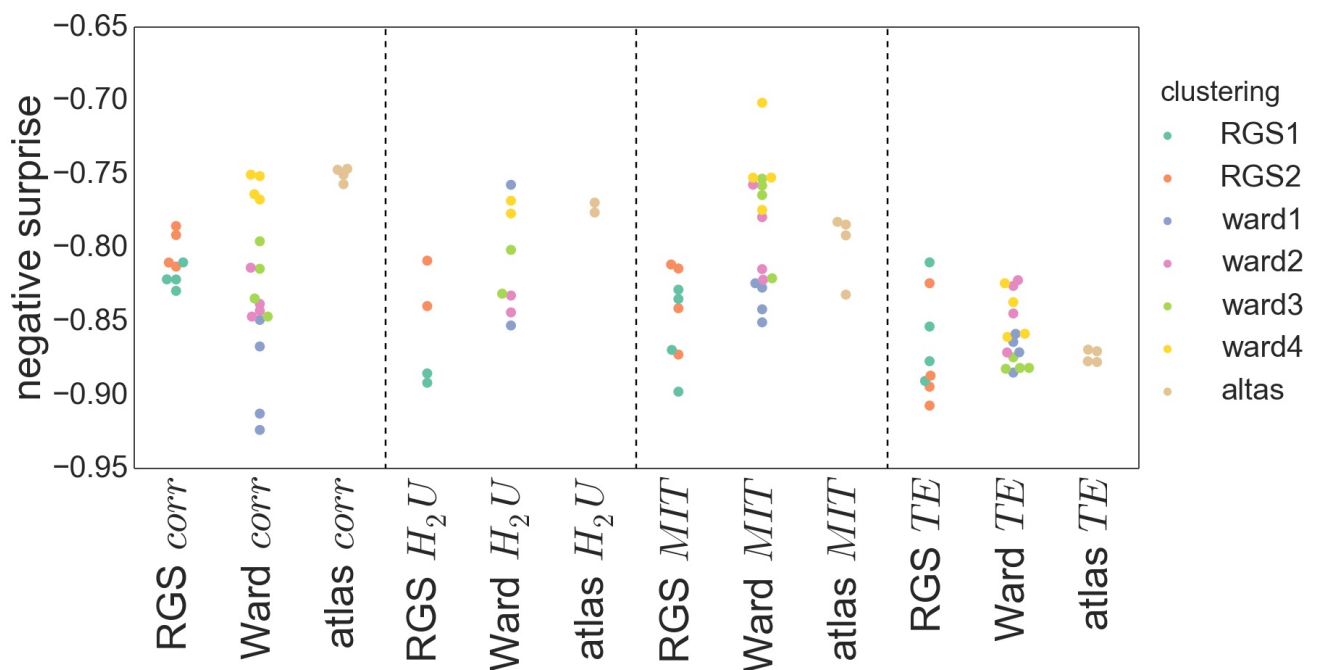
Figure S1: Negative surprise of the different graph construction methods. Figure identical with Fig.8 but with different clustering submethods depicted in different colors (see legend) .
