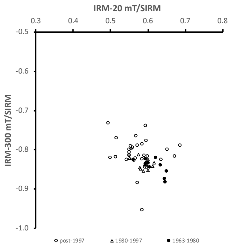
Supplementary Figure 3. Distinguishing combustion sources in sediments from Sky Pond (SKP1) using backfield isothermal remanent ratios (IRM-20 mT/SIRM and IRM-300 mT/SIRM), a variation of a magnetic bi-plot used to discriminate between fly ash and vehicular dusts (Hunt et al., 1984). SKP exhibits similar magnetic mineralogy throughout the core, with a slight shift to ‘harder’ antiferromagnetic minerals in the majority of post-1997 samples, characteristic of fly ash emissions (Hunt et al., 1984; Oldfield, 2014).
