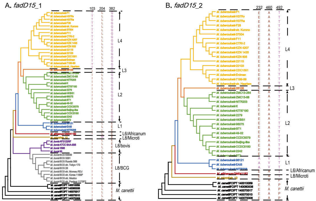
Supplementary Figure S14. The lineage-specific amino acid substitutions in fadD15_1 (A) and fadD15_2 (B) found in MTBC strains. Different colors indicate different MTBC lineage strains. The substituted amino acids are displayed in pink, and the corresponding STB controls are shown in brown.
