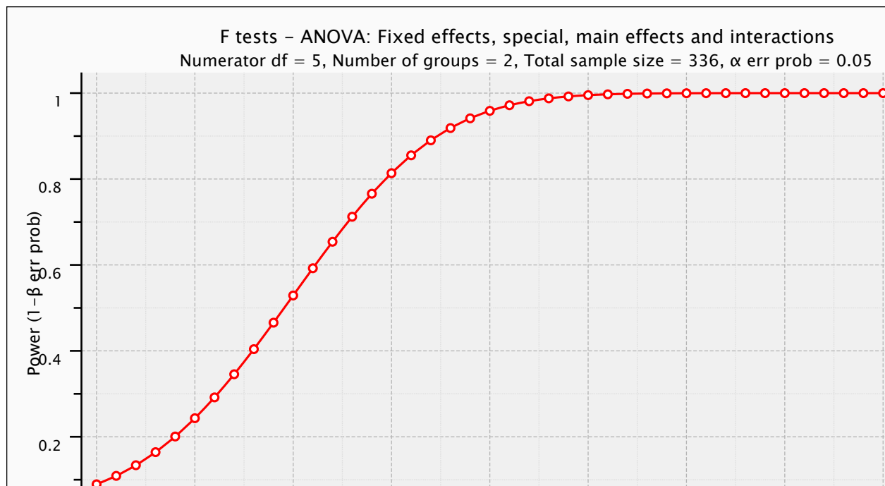
Supplementary Figure 2: The power of doing an eQTL analysis using ANOVA with an interaction term, calculated using G*POWER. This is a post hoc analysis of the power at various effect sizes, with a sample size of 336, type I error = 0.05, and 2 groups (male and female). The significance level is set at 0.05, and Number of groups (male vs female) set at 2.
