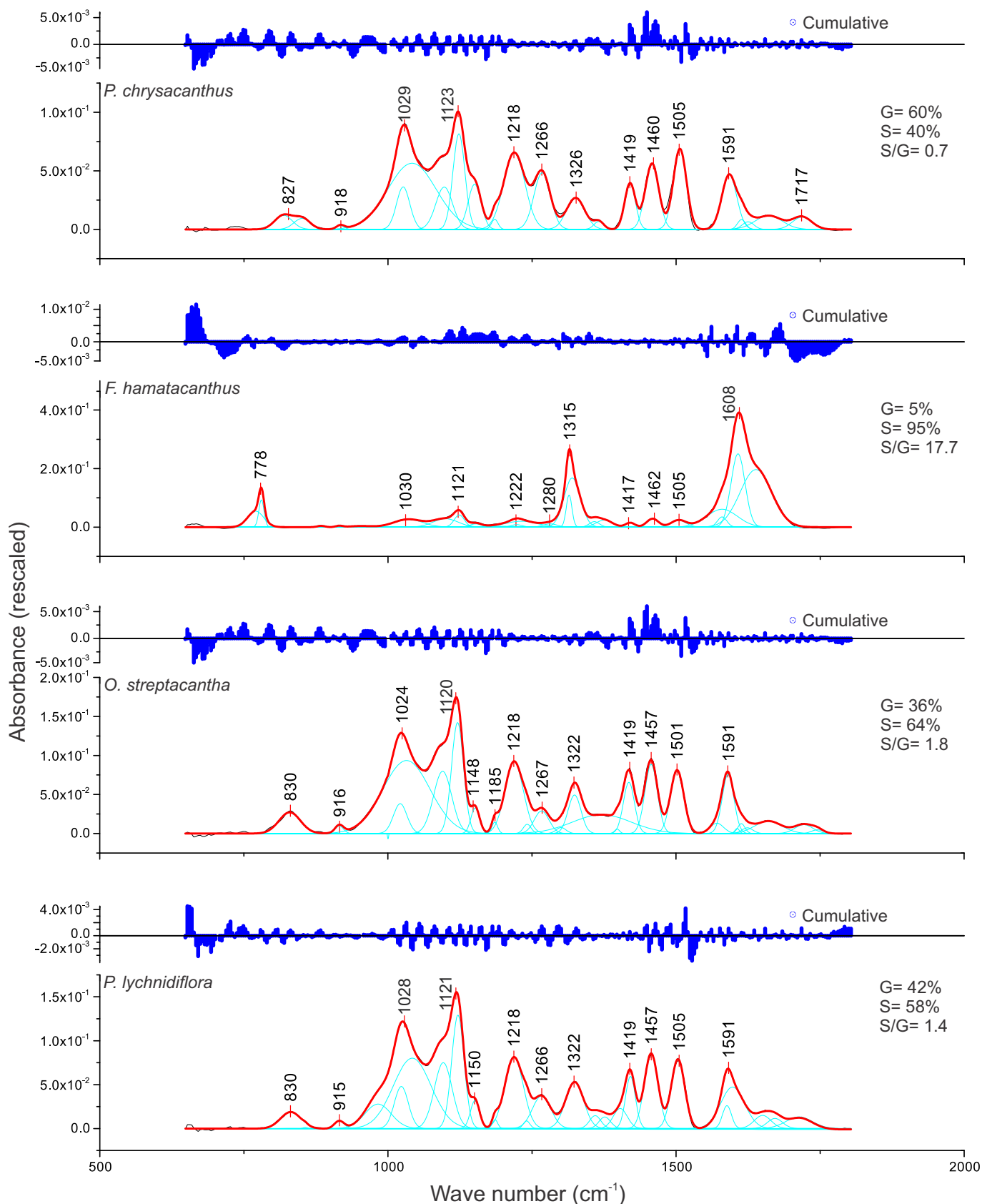
Figure S2. ATR-FTIR spectra deconvolution used to calculate relative abundances of G and S units, as well as the S/G ratio. The sum of the squares of the residual error for each spectrum was always in the range of \pm 5.0 \times 10^{-3} , the determination coefficients were never less than 0.98.
