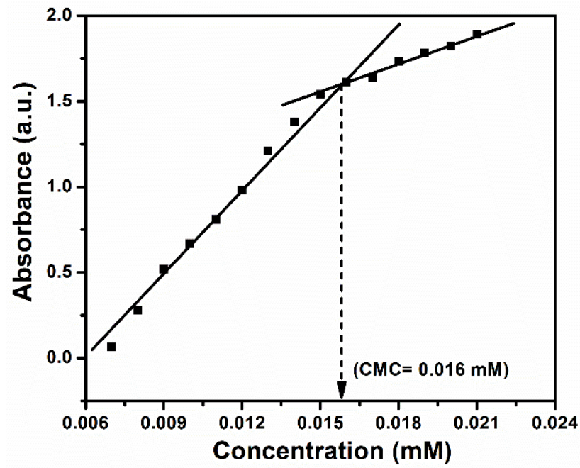
Figure S-1. Critical micelle concentration (CMC) of 2 -EB in water (at \lambda_{\text{max}} = 312 \text{ nm} )
