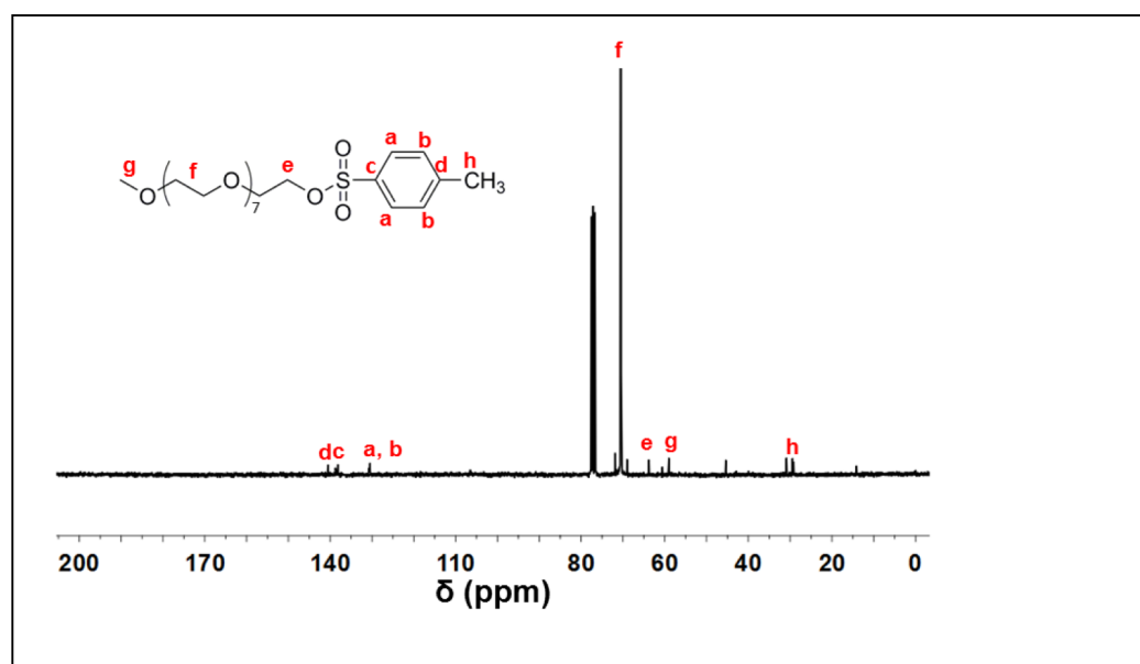
Figure S-8. 13 C NMR spectrum of tosylated- mPEG 350
