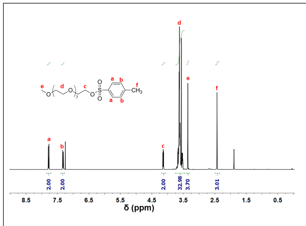
Figure S-7. 1 H NMR of tosylated-mPEG 350
