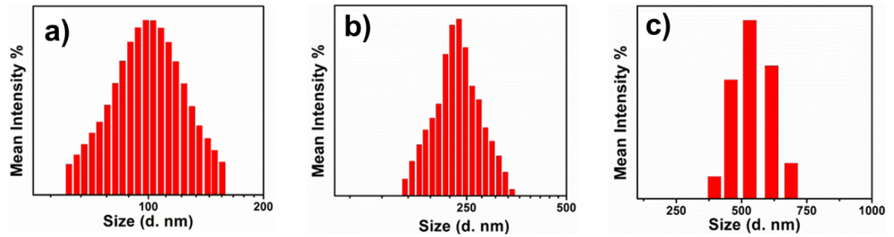
Figure S-2. Particle size distribution of 2 -LEB by DLS at different concentrations: 0.2 mg/mL (a), 1.0 mg/mL (b), 5.0 mg/mL (c).
