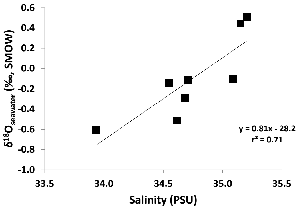
Supplementary Figure S1. Linear relationship between sea surface salinity and \delta^{18}\text{O}_{\text{sw}} in NW Australian coastal waters.
