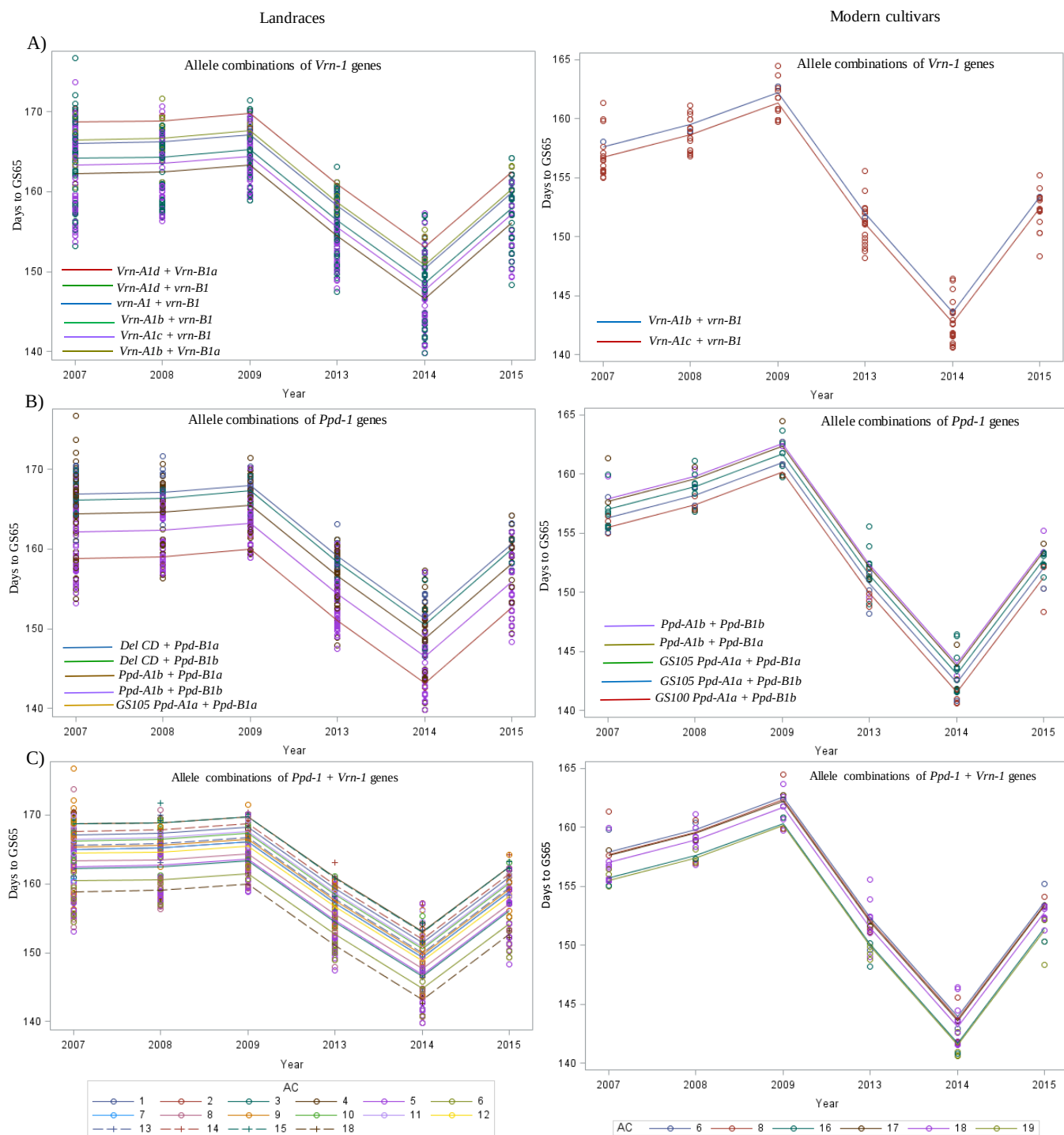
SUPPLEMENTARY FIGURE S3. Allele combinations x year interaction for the number of days to GS65 (anthesis) in landraces (left) and modern cultivars (right). A) Allele combinations of Vrn-1 genes; B) Allele combinations of Ppd-1 genes; C) Allele combinations of Vrn-1 + Ppd-1 genes. See Table 6 for the meaning of allele combination (AC) numbers.
