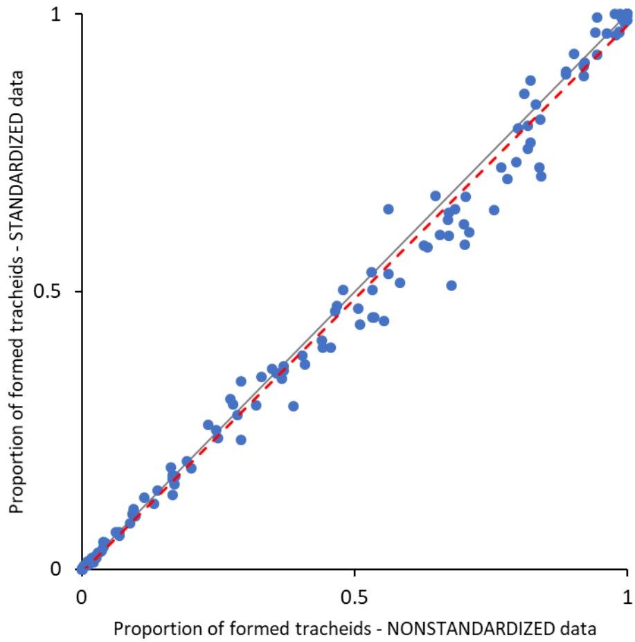
Figure S4: Relationship between proportion of tracheids in enlarging, wall-thickening and mature phases formed during individual dates of xylogenesis monitoring based on standardized and nonstandardized data. Red dashed line represents least-square regression.
