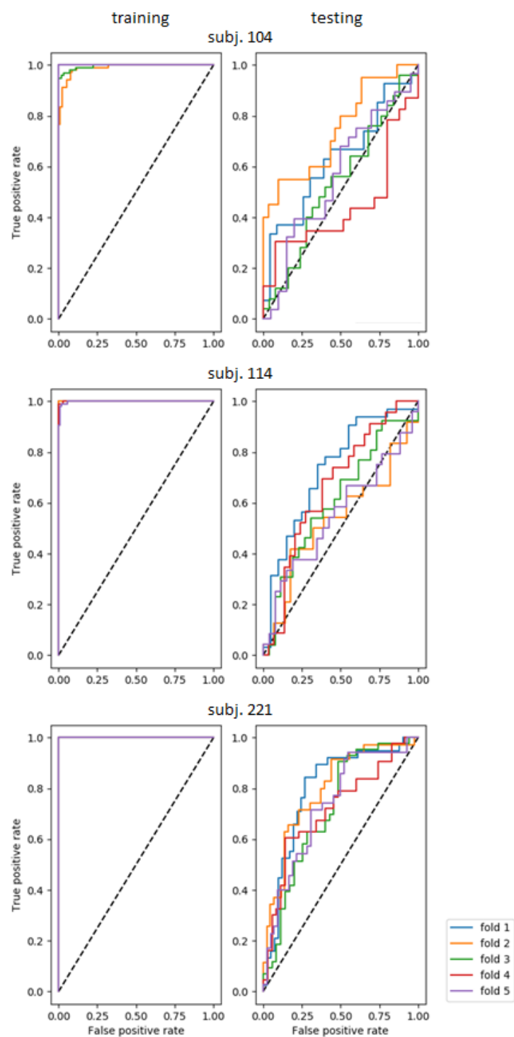
Supplementary Figure 1. ROC AUC curves for each fold of training (left) and testing (right) procedures, obtained on datasets of three subjects. Some lines may not be visible if they coincide with lines drawn on top of them.
