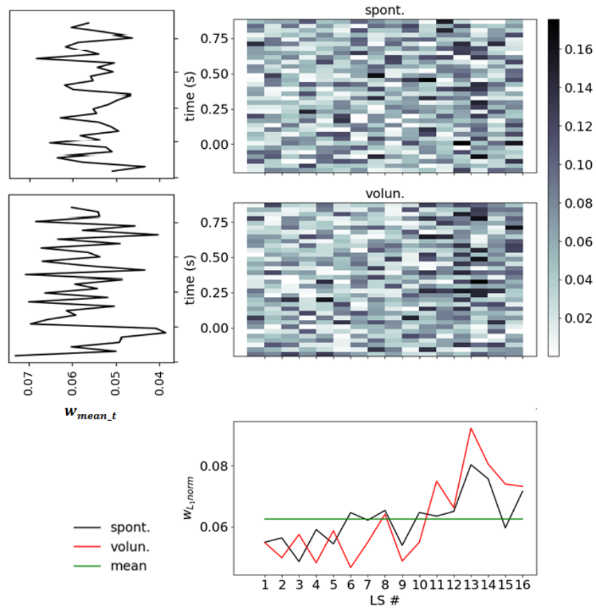
Supplementary Figure 2. Output weights of LF-CNN learned on participant 114 data in time interval -0.2 ... 1.0 s for spontaneous and voluntary classes (top and middle, respectively), LS' weights for each class according to Equation 4, where proportion of the L1-norm of output weights over time points in total sum of L1-norms of all LSs (bottom), averaged weights in every time point over all LSs (left).
