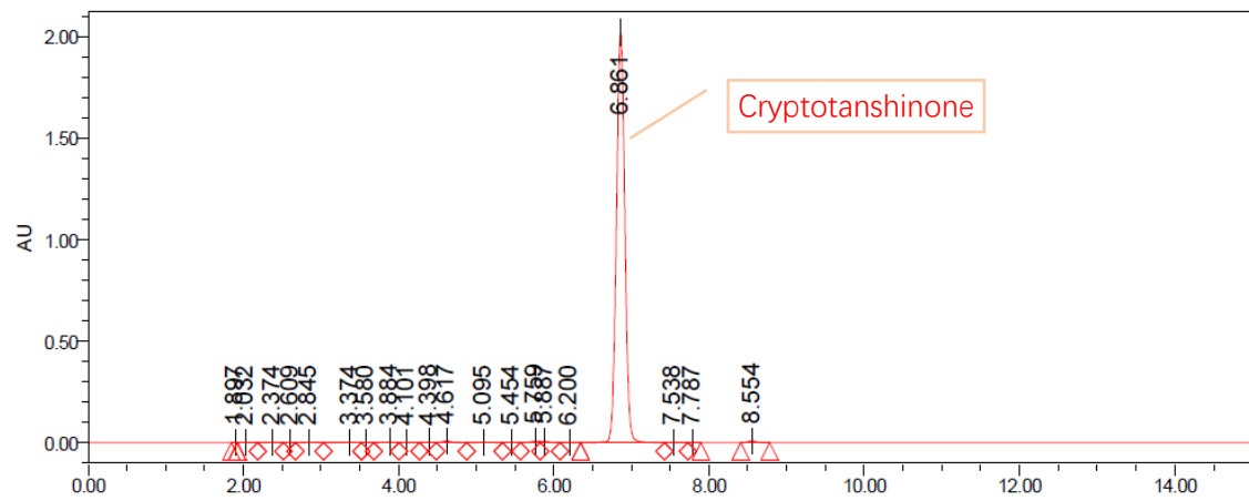
Fig.S3 A. the chemical structure of cryptotanshinone; B. the HPLC chemoprofile of cryptotanshinone.
