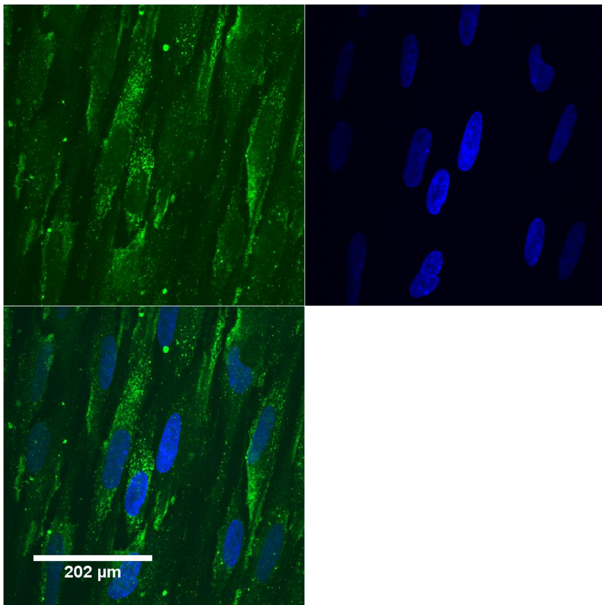
Figure S1: Confocal microscopy: perivascular marker VAP-1 (green) on cell surface of SUSD2 + cells. Image taken at 60 x magnification using a Zeiss Laser Scanning Microscope LSM 510. Nuclei visualized with DAPI (blue). Scale bar represents 202μm.
