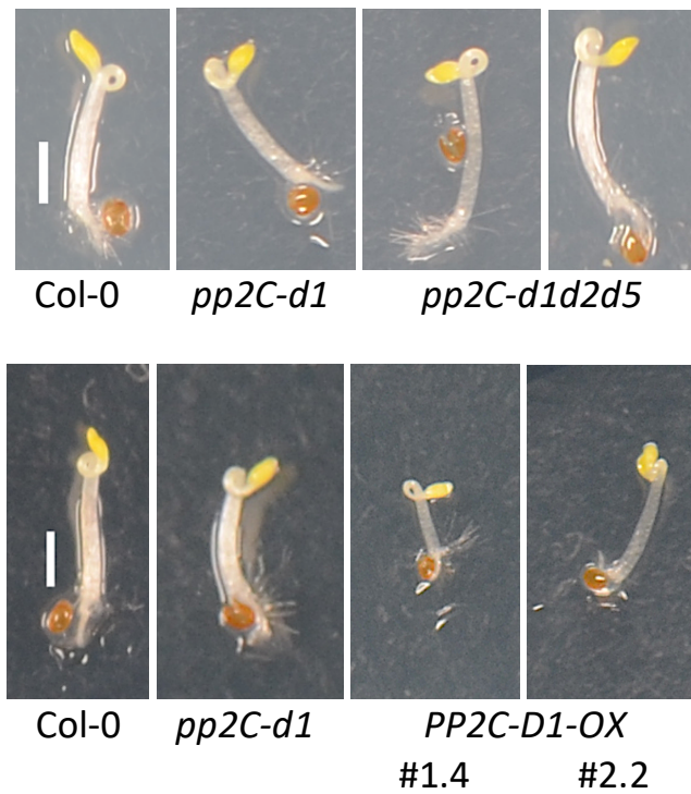
Supplementary Figure S1. ACC-induced hook curvature in PP2C.D mutants. Visual phenotypes of 3-day-old (Top) and 4-day-old (Bottom) etiolated Col-0, pp2c-d1 , pp2c-d1d2d5 and PP2C-D1-OX seedlings grown in the dark on MS medium containing 2 \mu M ACC. Bar = 1 mm.
