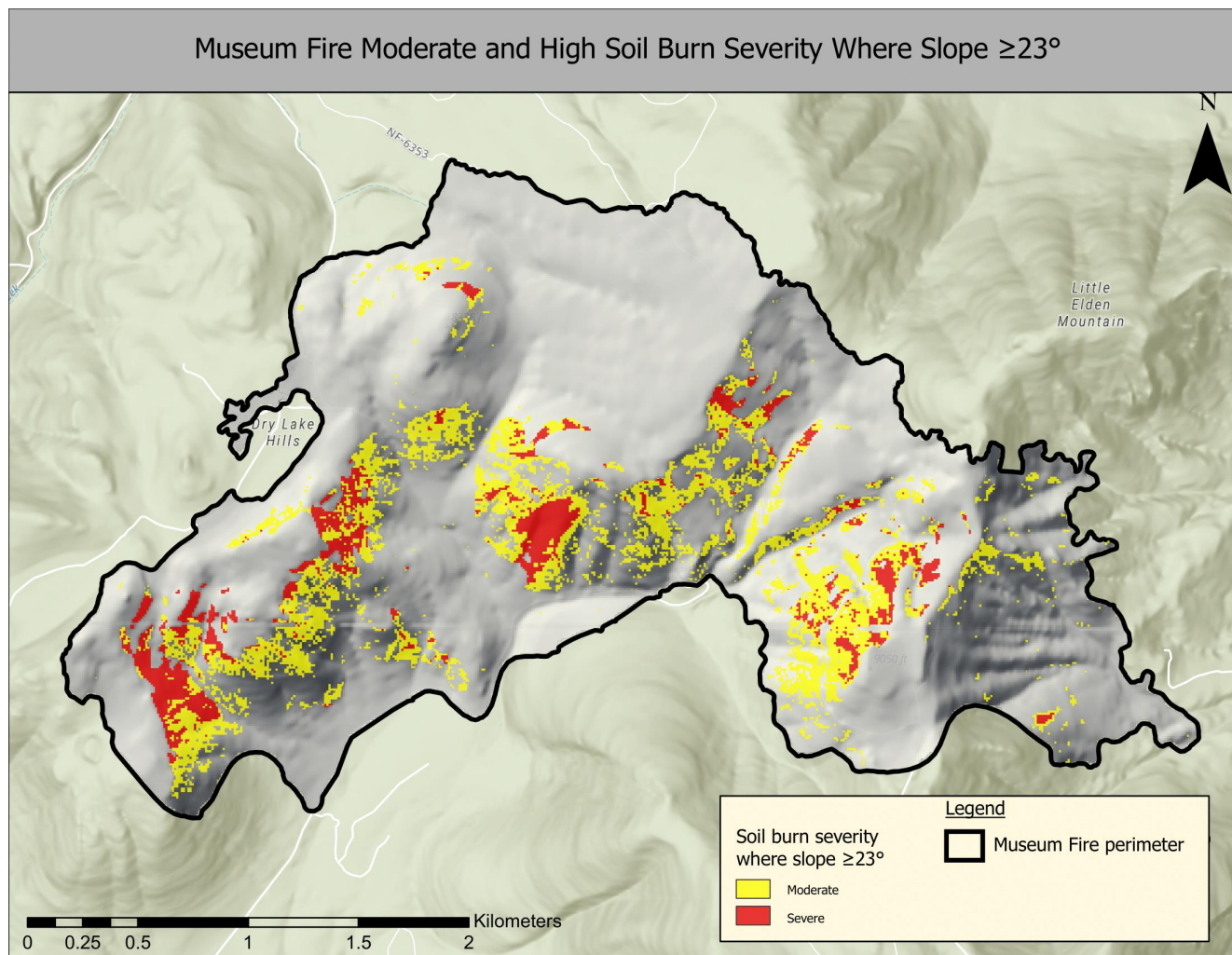
Figure S1: Museum Fire burn scar where moderate and severe soil burn severity intersect with slope angles \geq 23^\circ , representing where there is higher post-fire debris flow probability.
