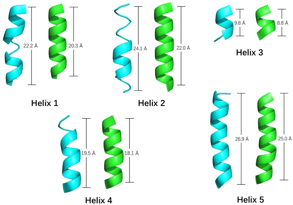
Supplementary Figure 2. The comparison of helix regions from the packed state (blue) and free state (green). The start and end residues of helices were defined according to the free state conformation. The spatial length of helices was measured by the distance between C \alpha of the two terminal residues.
