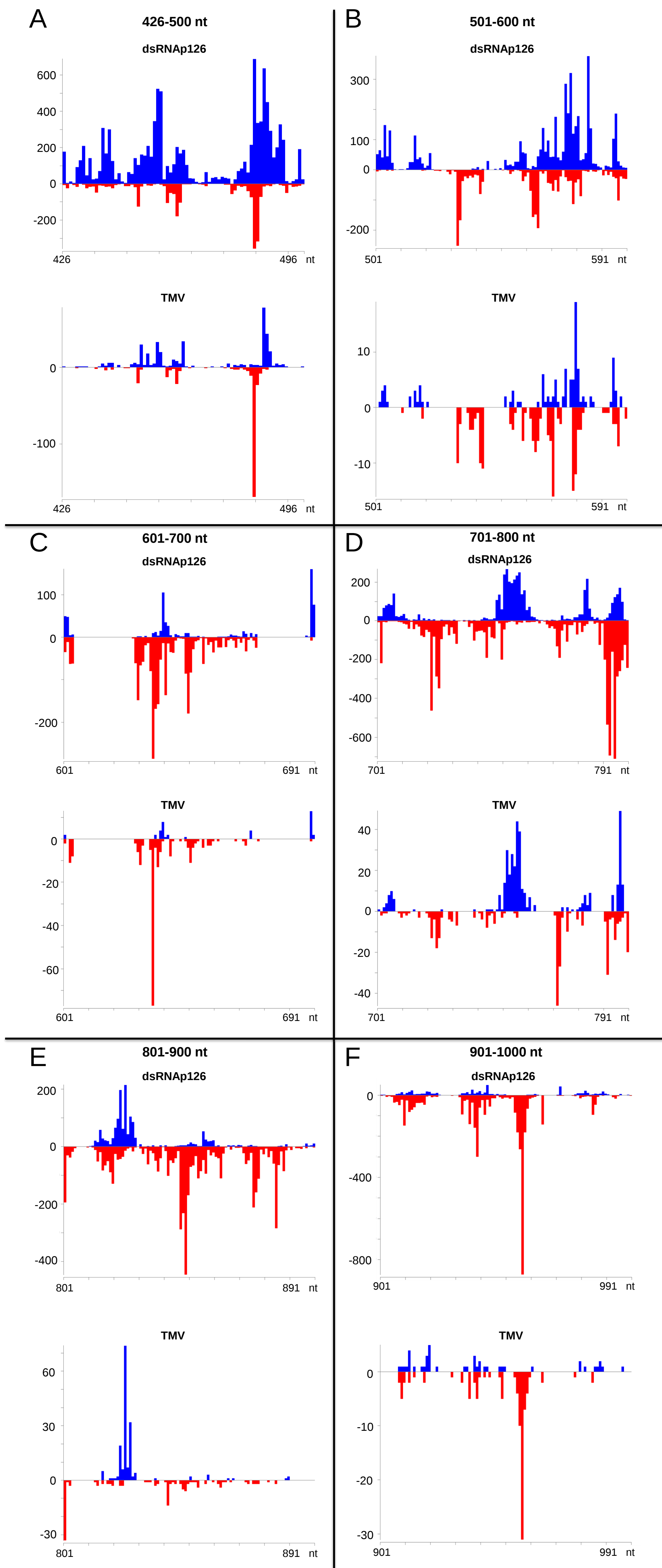
FIGURE S3 | Similar pattern of dsRNAp126-derived and TMV-derived siRNA production in dsRNAp126 and TMV treatments, respectively. SiRNAs produced from region 426-500 nt (A) , 501-600 nt (B) , 601-700 nt (C) , 701-800 nt (D) , 801-900 nt (E) , and 901-1000 nt (F) . The numbers derive according to the virus genome.
