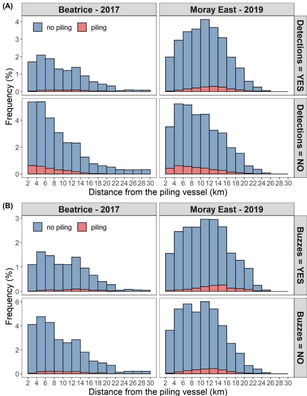
Supplementary Figure 6 Frequency distribution of the distance from the piling vessel (km) during (in red) and outside (in blue) piling hours, in presence-absence of harbour porpoise echolocation click detections (A) and buzzing activity (B) , between 2017 and 2019 at the Beatrice and Moray East offshore windfarms
