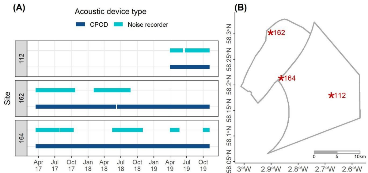
Supplementary Figure 1 (A) Passive Acoustic Monitoring timeline at three long-term monitoring sites to detect echolocation clicks with CPODs (in dark blue) and record underwater broadband noise levels with noise recorders (in light blue) (B) Noise recorders locations (in red) within the two offshore windfarms (grey line)
