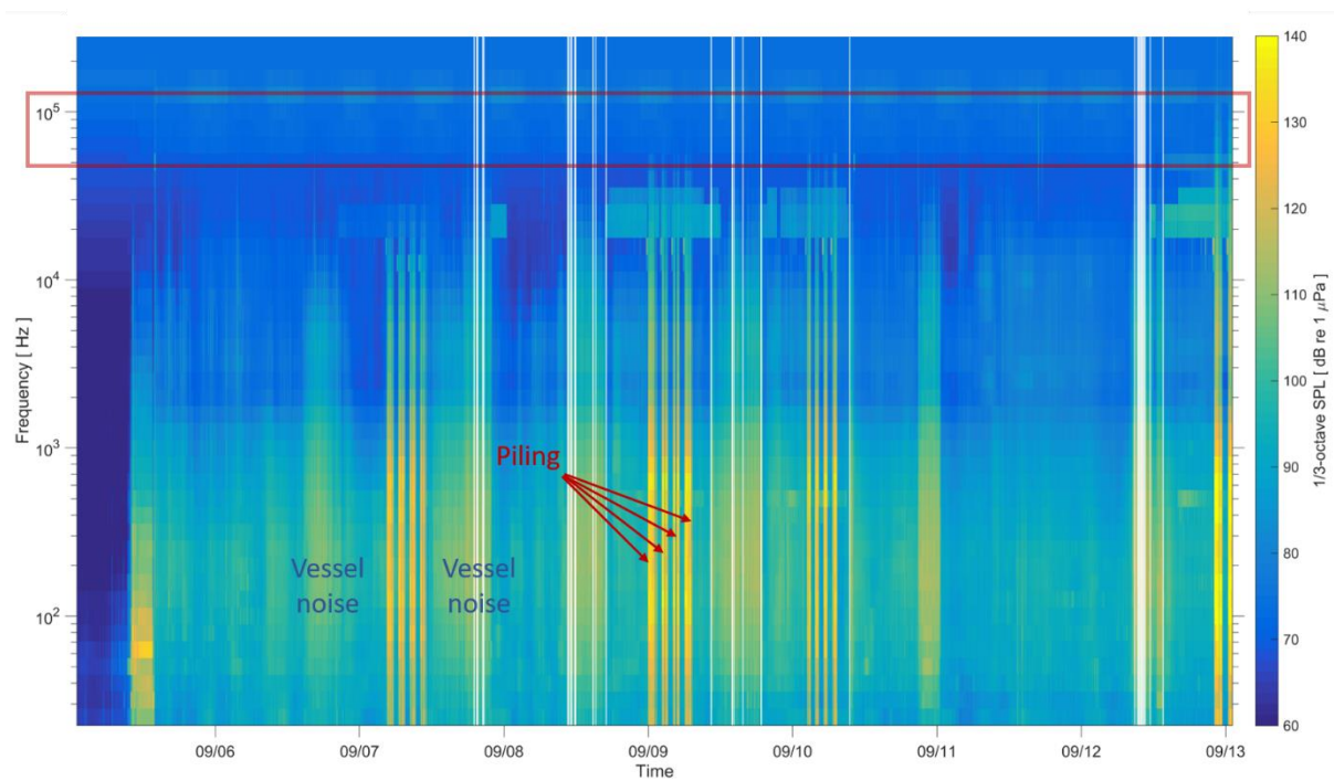
Supplementary Figure 10 1/3 octave band spectrogram to highlight variability in noise levels between 5 and 13 September 2017 at Beatrice offshore windfarm, 60-s resolution; at high frequencies (red box) both piling and vessel noise are below ambient noise levels.
