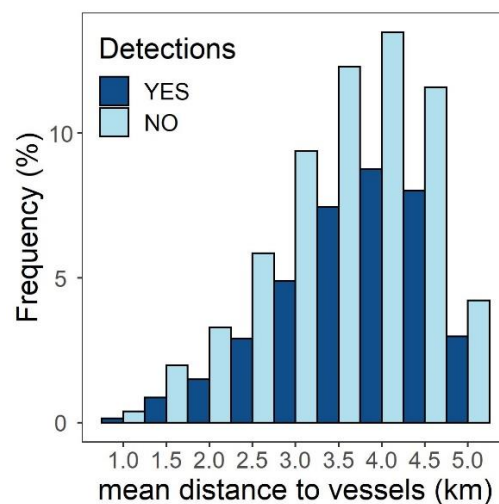
Supplementary Figure 8 Frequency distribution of the mean distance between any vessels and each CPOD per hour, in presence (dark blue) or absence (light blue) of harbour porpoise echolocation click detections between 2017 and 2019 at the Beatrice and Moray East offshore windfarms
