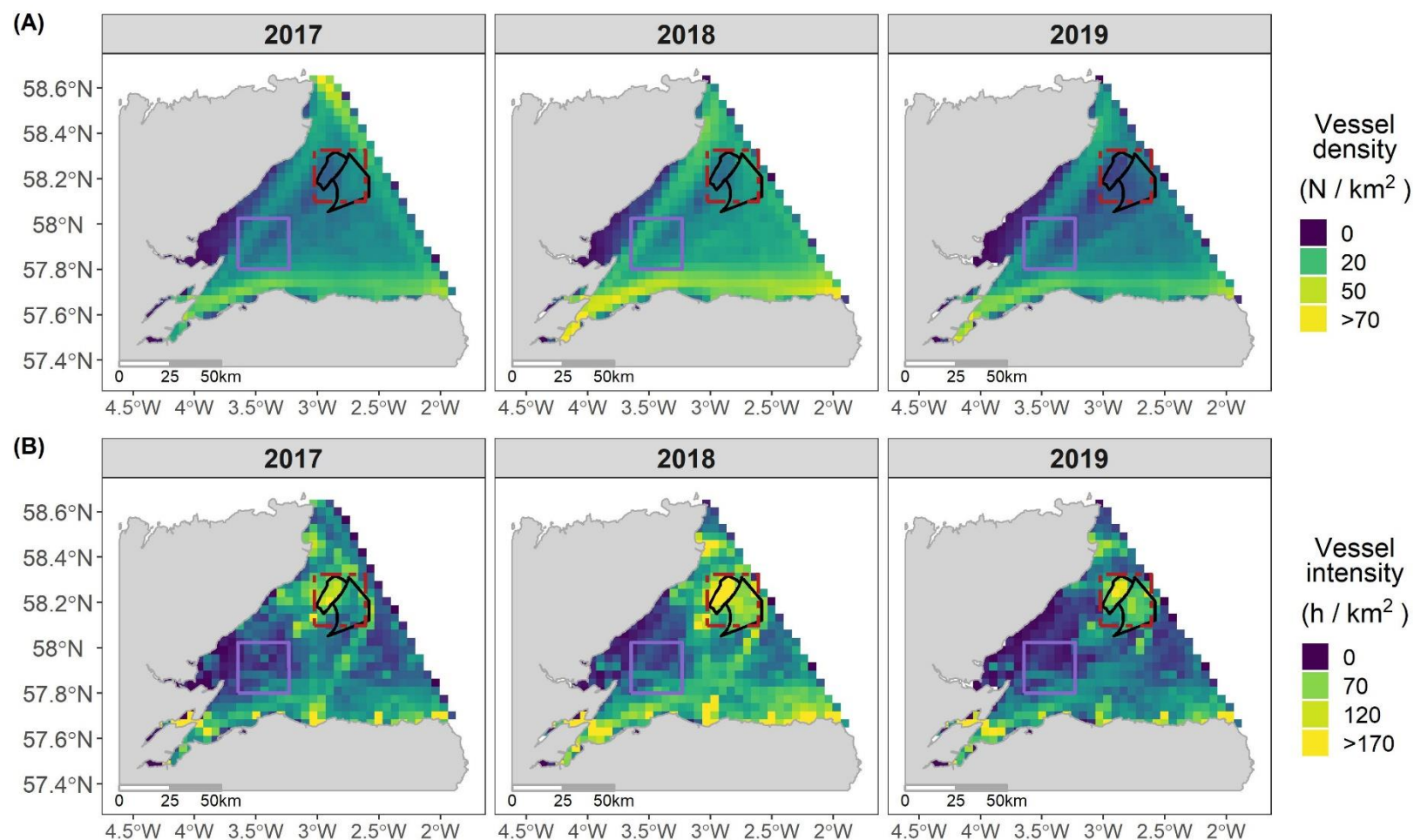
Supplementary Figure 5 Vessel density (A) and intensity (B) in the Moray Firth (4 x 4 km grid) between 2017 and 2019; the Beatrice and Moray East offshore windfarms are represented in black in the impact block (dashed red line) and the reference block is in purple.
