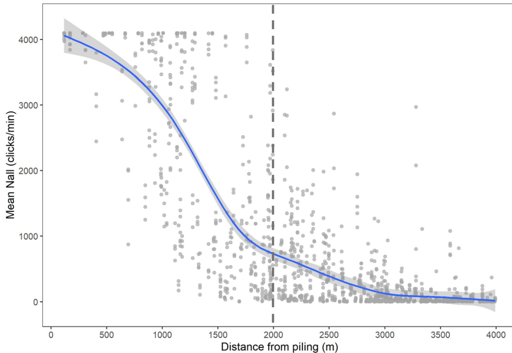
Mean Nall during all piling events in 2017 (02/04-02/12/2017) from 36 deployments and 30 sites
