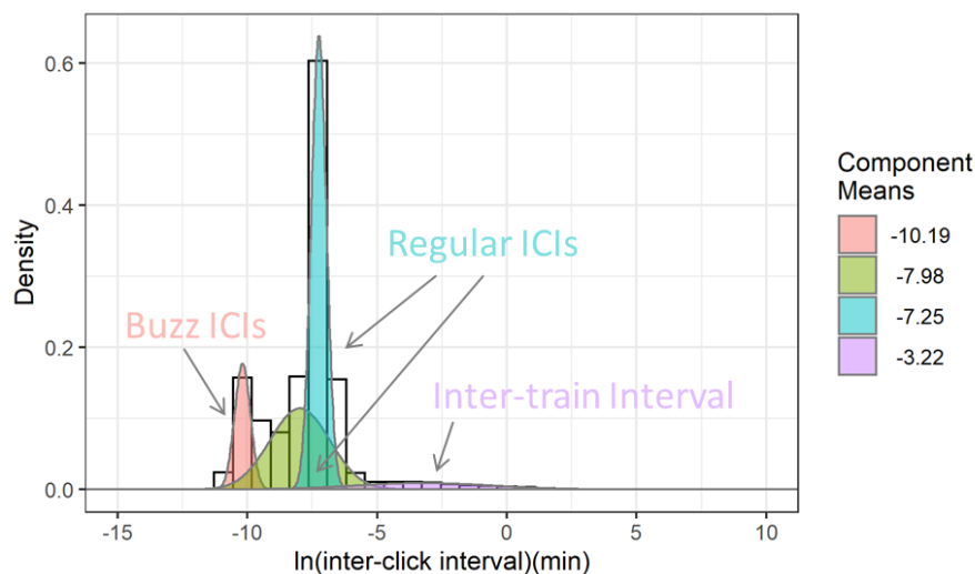
Supplementary Figure 3 Example of the results of a Gaussian mixture model using four components for one CPOD Inter-Click Interval (ICI) time series, following Pirotta et al. (2014). The buzz ICIs are represented in pink, the regular ICIs in blue and green, the inter-train intervals in purple. The x-axis represents the natural logarithm of the ICIs in minutes.
