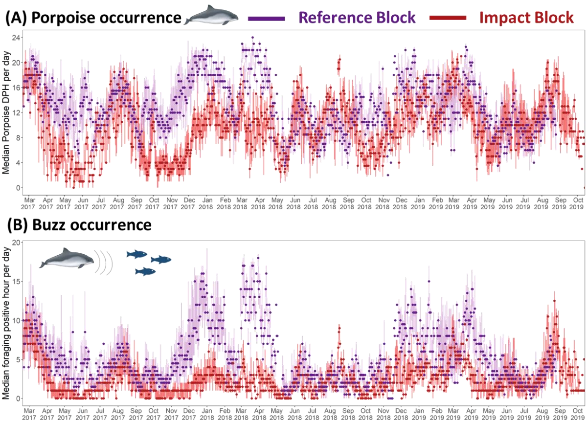
Supplementary Figure 4 Median harbour porpoise (A) detections per hour (DPH) and (B) foraging positive hours per day within the reference (in purple) and impact (in red) blocks between March 2017 and October 2019; the dots represent the median and the lines represent the first and third quantile
