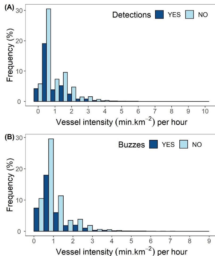
Supplementary Figure 7 Frequency distribution of the vessel intensity (min/km 2 ) per hour, in presence (dark blue) or absence (light blue) of harbour porpoise echolocation click detections (A) and in presence (dark blue) or absence (light blue) of buzzes (B) , between 2017 and 2019 at the Beatrice and Moray East offshore windfarms
