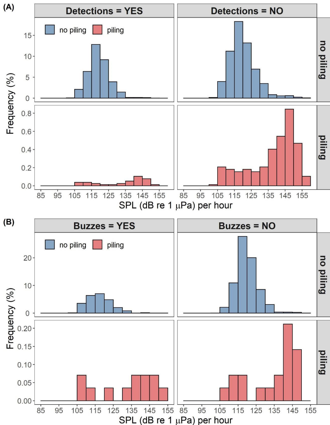
Supplementary Figure 9 Frequency distribution of the broadband sound pressure level (SPL) per hour during (in red) and outside (in blue) piling hours, in presence-absence of harbour porpoise echolocation click detections (A) and buzzing activity (B) , between 2017 and 2019 at the Beatrice and Moray East offshore windfarms
