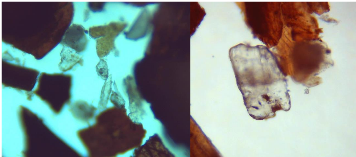
Figure S1: Photos of struvite obtained in the bioreactors with an optical microscopy at 25x
