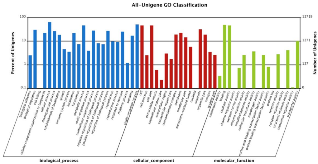
Figure S1 GO classification analysis of Unigenes in All-Unigene. GO functions is showed in X-axis. The right Y-axis shows the number of genes which have the GO function, and the left Y-axis shows the percentage.
