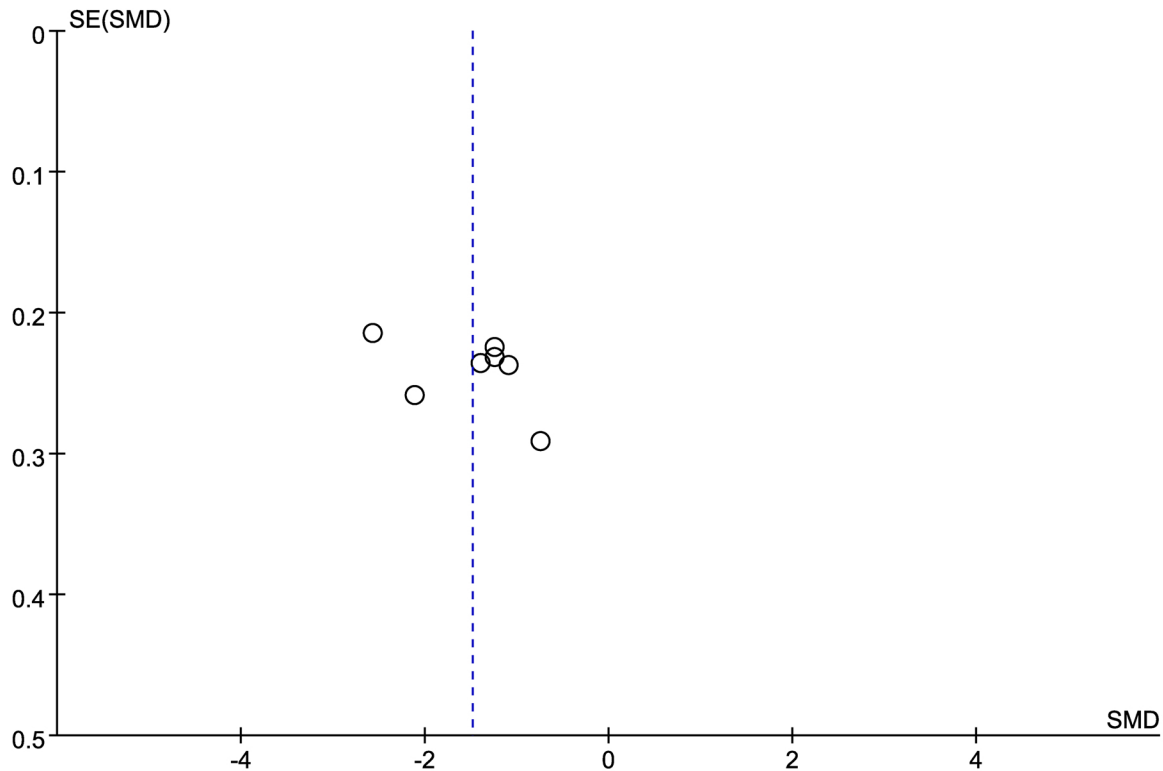
Figure S11: Funnel plot of psychiatric symptoms
