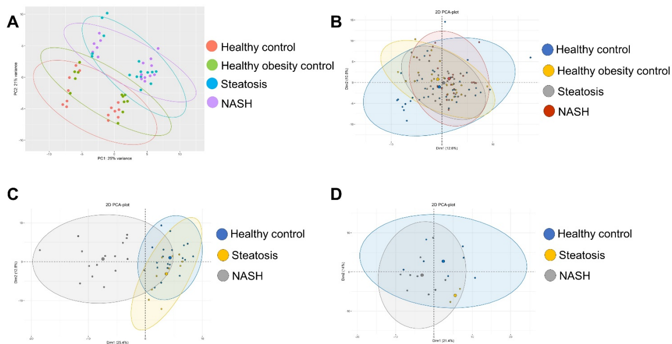
Supplementary Figure 1. PCA plots for: A) Suppli et al. [29], B) Horvath et al. [31], C) Lake et al. [30], D) Frades et al. [25].
