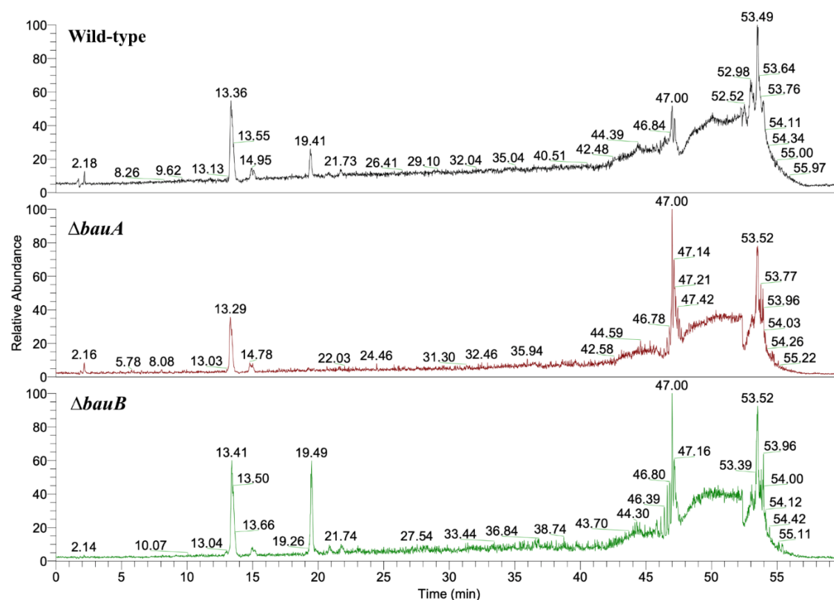
Supplementary Figure 13. Comparison between the total ion current (TIC) chromatographic profiles of the ABHL5 fractions of A. baumannii wild-type and mutant strains lacking genes involved in the influx of acinetobactin.
