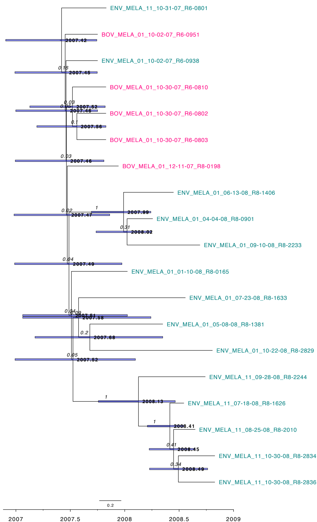
Supplementary Figure S8. Rooted, time-scaled maximum clade credibility (MCC) phylogeny constructed using core SNPs identified among 19 Salmonella Meleagridis genomes isolated from subclinical bovine sources (pink tip labels) and the surrounding bovine farm environment (teal tip labels). Branch labels (black italic text) denote posterior probabilities of branch support, while node labels (black boldfaced text) denote node ages. Time in years is plotted along the X-axis, and branch lengths are reported in years. Node bars denote 95% highest posterior density (HPD) intervals for common ancestor (CA) node heights. Core SNPs were identified using Snippy. The phylogeny was constructed using the results of ten independent runs using a strict clock model, the Standard TPM2 nucleotide substitution model, and the Coalescent Bayesian Skyline population model implemented in BEAST version 2.5.1, with 10% burn-in applied to each run. LogCombiner-2 was used to combine BEAST 2 log files, and TreeAnnotator-2 was used to construct the phylogeny using CA node heights.
