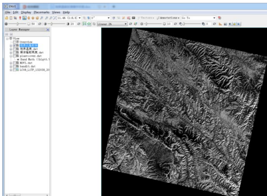
Fig.5. Surface Specific Emissivity
