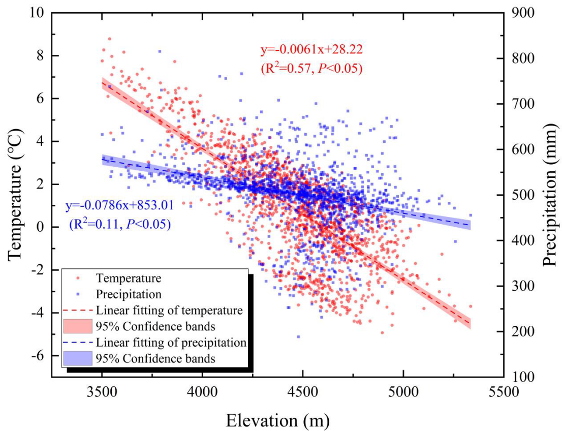
Supplementary Figure 1. Variation of climatic factors with altitude
