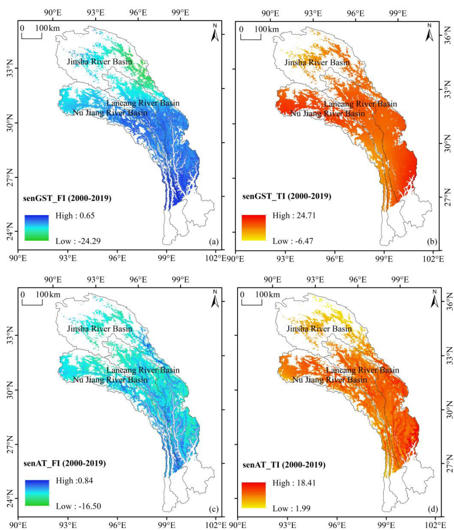
Supplementary Figure 4. The trends of long-term averaged freezing/thawing index in the past 20 years.
