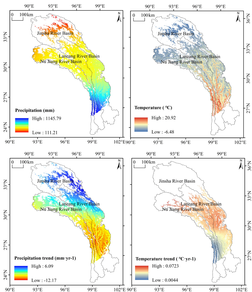
Supplementary Figure 2. Multi-year spatial patterns and trends of climate factors (2000-2019)
