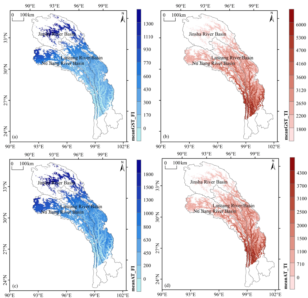
Supplementary Figure 3. The spatial distribution of long-term averaged freezing/thawing index during 2000-2019. ((A)-(D) represent the ground surface freezing index(GFI), ground surface thawing index(GTI), air temperature freezing index(AFI), and air temperature thawing index(ATI), respectively.)
