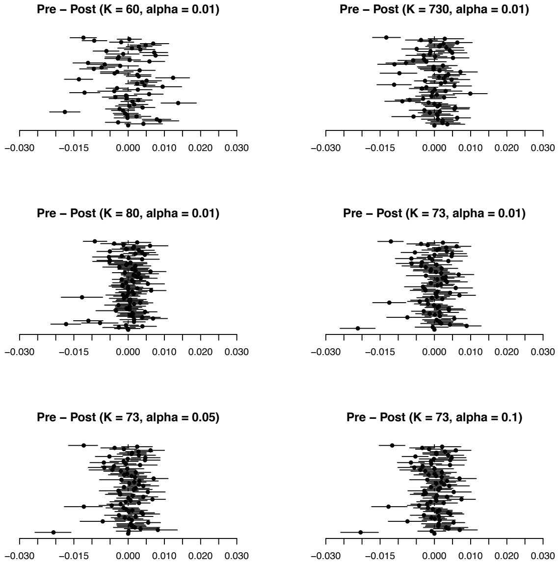
Appendix Figure 4: Topic and Alpha STM Optimization
