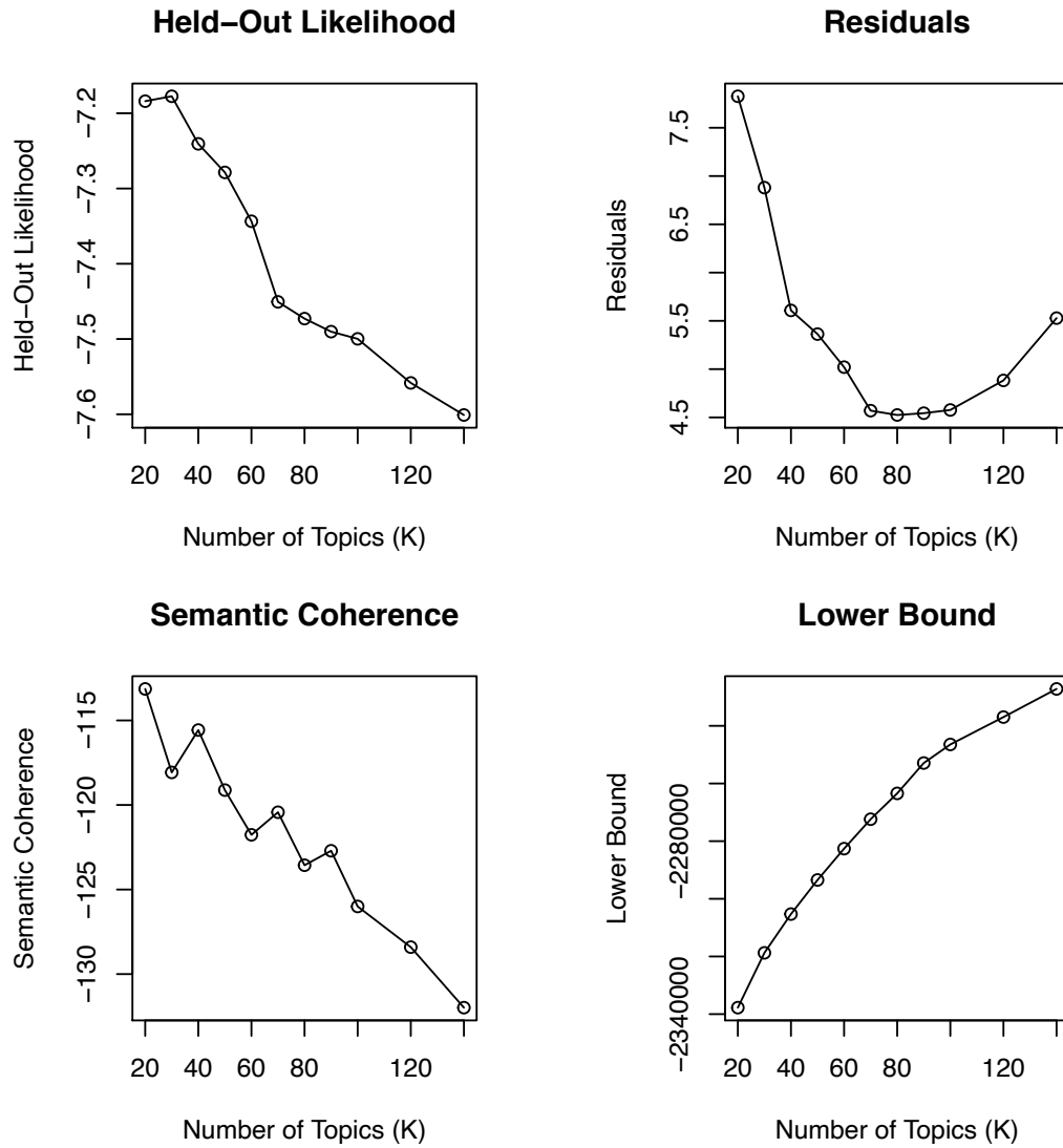
Appendix Figure 3: STM Optimization of Topics
