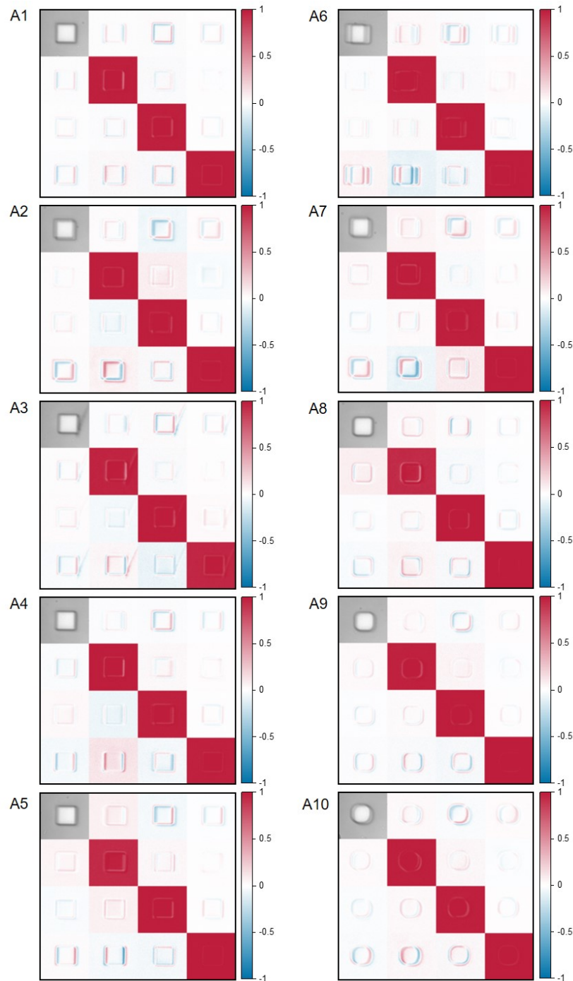
Figure S1. Mueller matrix images of structures in row A, not drift corrected.
