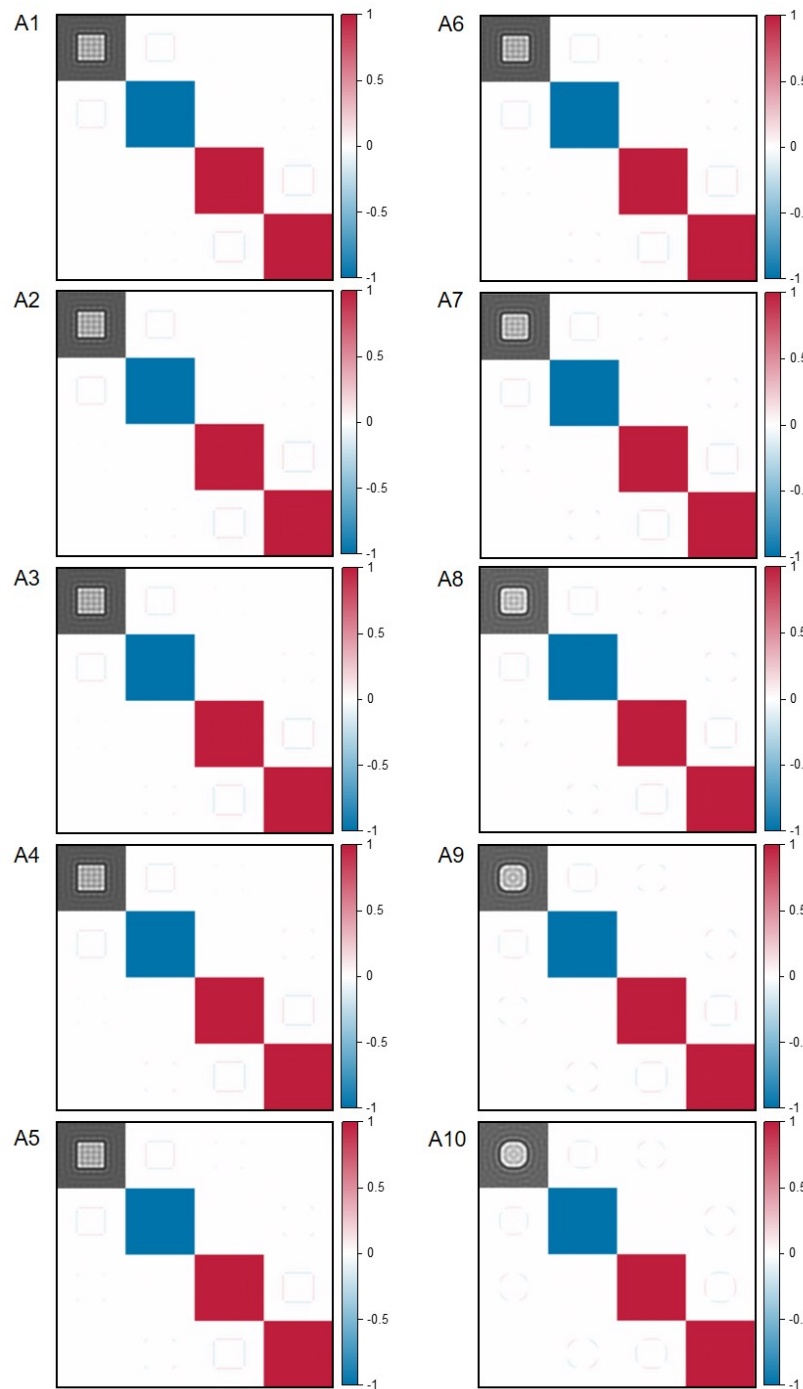
Figure S3. Mueller matrix images of structures in row A, simulated.
