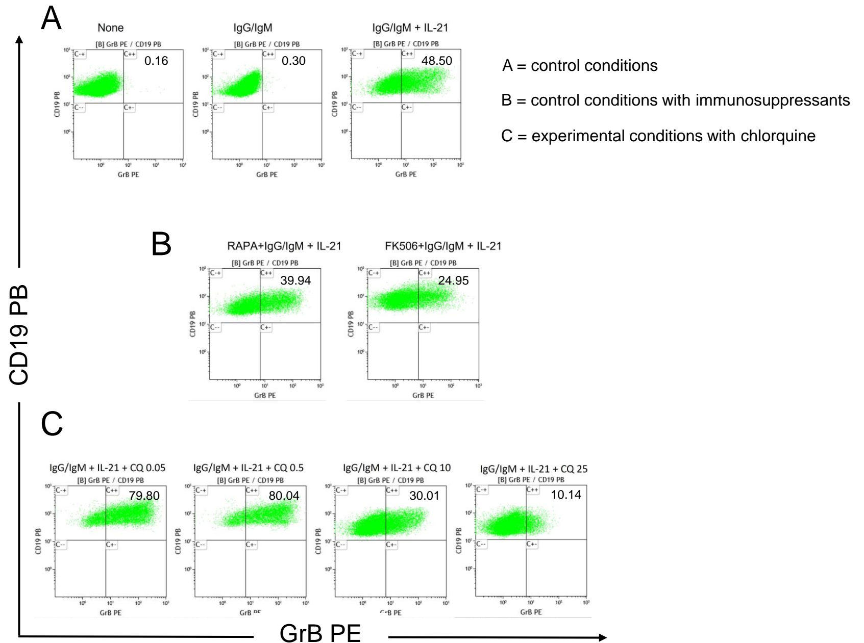
Figure S1. Effect of CQ on GrB producing regulatory B-cells: Representative flow cytometric data.
