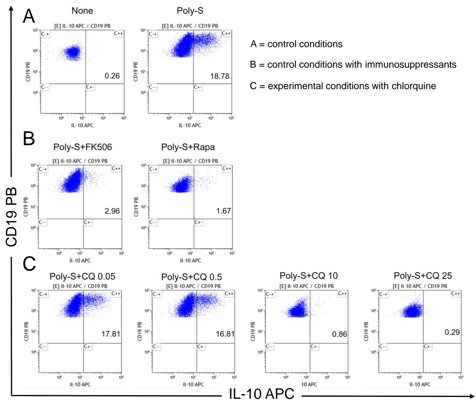
Figure S2. Effect of CQ on IL-10 producing regulatory B-cells: Representative flow cytometric data.
