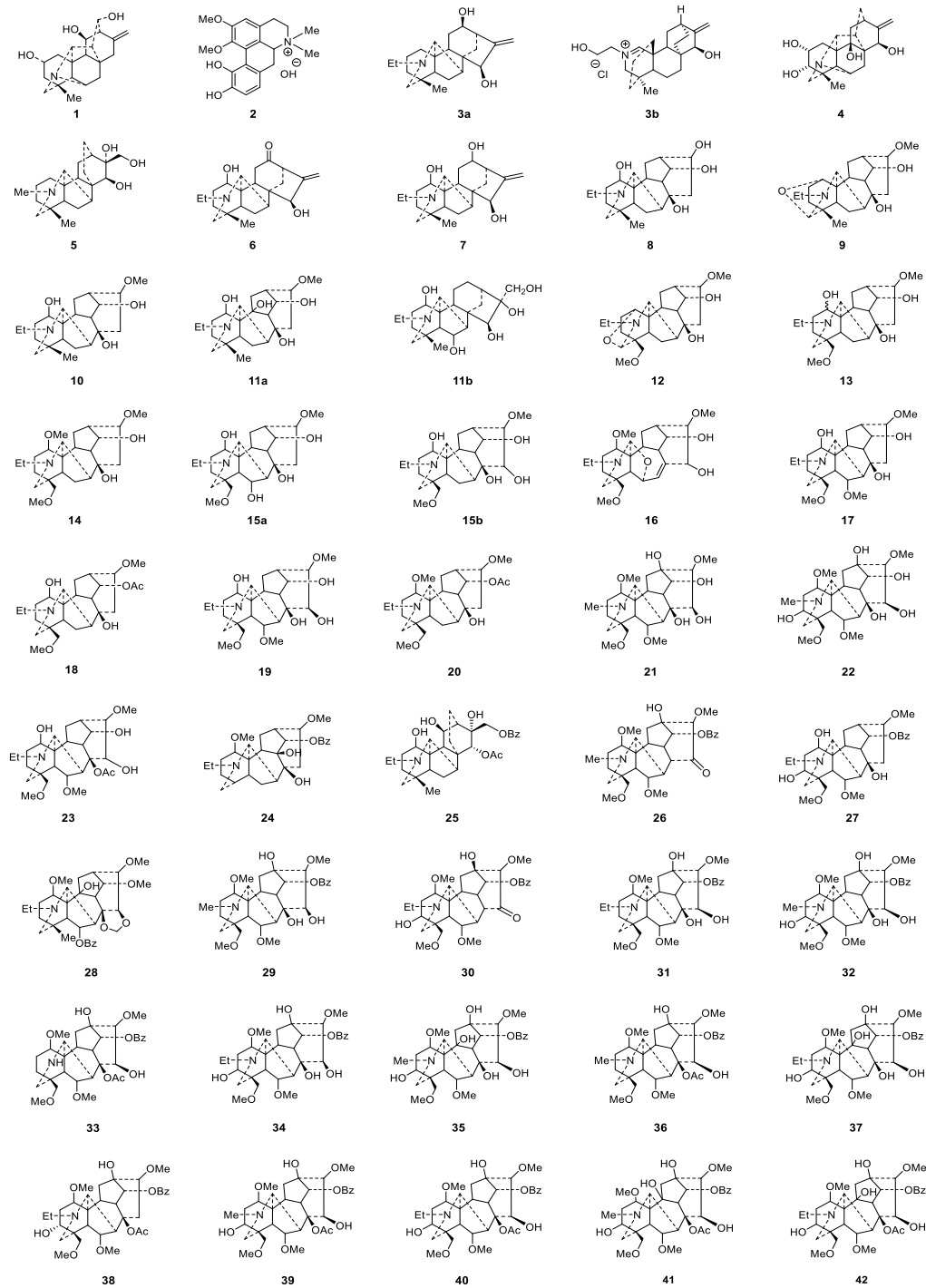
Supplementary Figure S2. Chemical structures of 42 metabolic markers of raw and processed Fuzi steamed for 0, 4.0 and 8.0 h.
