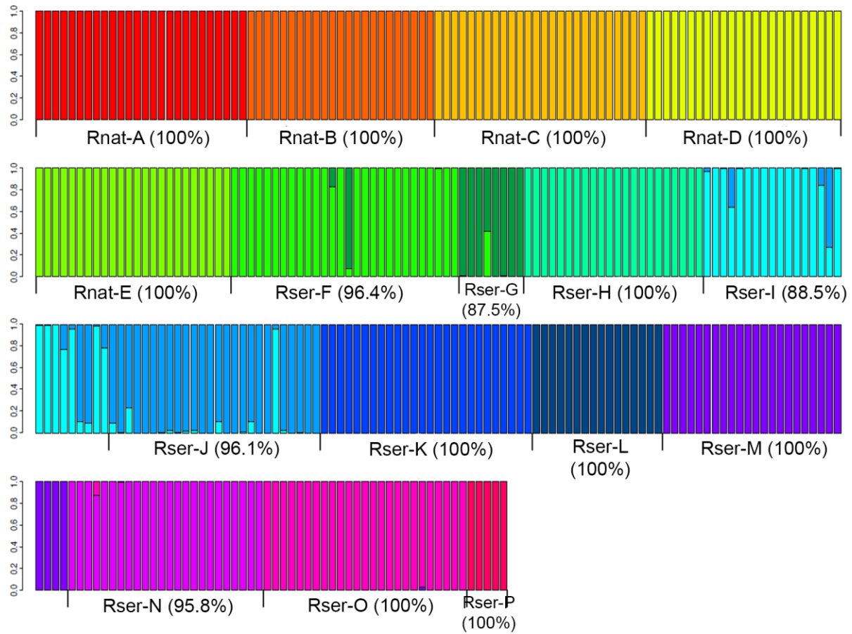
Supplementary Figure 2. Histogram of assignments of individuals to monospecific populations of R. nathaliae and R. serbica . Population codes the same as in Table 1. The assignment posterior probability (expressed in %) is given in brackets for each population.
