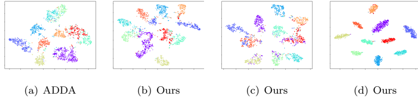
Figure 1: t -SNE plot of the feature domains for MNIST→USPS.
