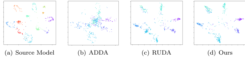
Figure 2: t -SNE embeddings of the representations for Syn12→Real6. The features are embedded into the same subspace and visualized within the same scope. (a) is the learnt source representation with 12 classes. (b)(c)(d) are the adapted target representation with 6 classes. The representation from our method consists of 6 disentangled clusters, while others tend to be more entangled or contains excessive number of clusters.
