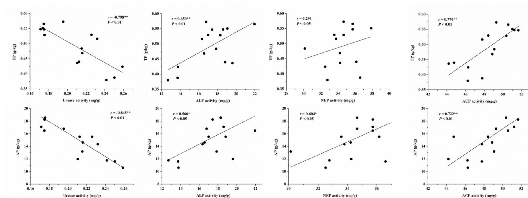
FIGURE S1 | The relationship between the soil enzymatic activity and TP, AP. *, ** respectively indicated P < 0.05 , P < 0.01 . TP, total phosphorus; AP, available phosphorus; ACP, acid phosphatase; NEP, neutral phosphatase; ALP, alkaline phosphatase.
