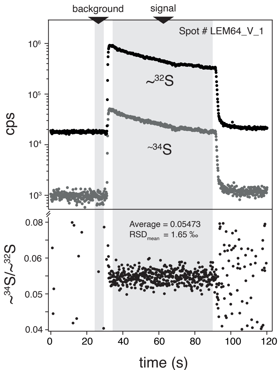
Data Sheet 1: Example of a LA-ICP-MS spot analysis of pyrite analyzed in this study. Sulfur isotopes are measured in mass shift mode as ^{34}\text{S}^{16}\text{O}^+ and ^{32}\text{S}^{16}\text{O}^+ denoted \sim^{34}\text{S} and \sim^{32}\text{S} , respectively. Integration windows for background and signal are indicated, such as the resulting background corrected \sim^{34}\text{S}/\sim^{32}\text{S} ratios. For further details see methods section.
