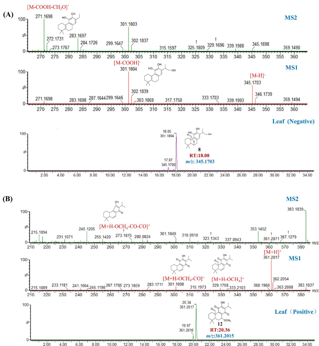
Supplementary Figure 1. The MS/MS fragment patterns of compound 9 and 12. (A) MS/MS fragment patterns of compound 9 in both negative-mode. (B) MS/MS fragment patterns of compound 12 in positive-ion mode. Compounds 9 and 12 are examples of all compounds.
