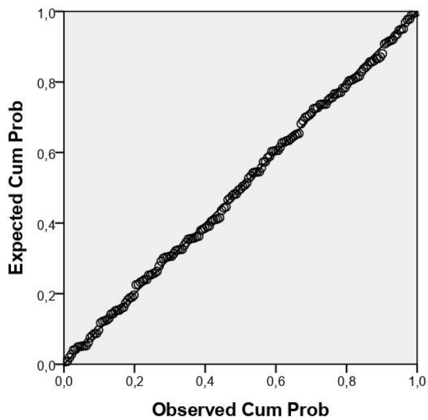
Supplementary Figure 8. Normal P-P plot of regression standardized residual for psychological well-being.
