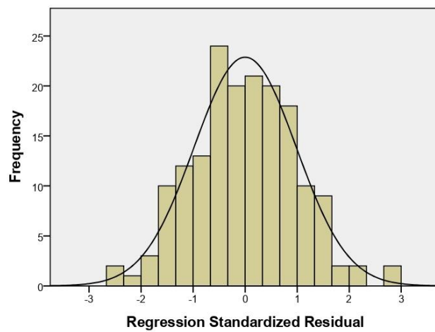
Supplementary Figure 4. Histogram of regression standardized residual for psychological well-being.
