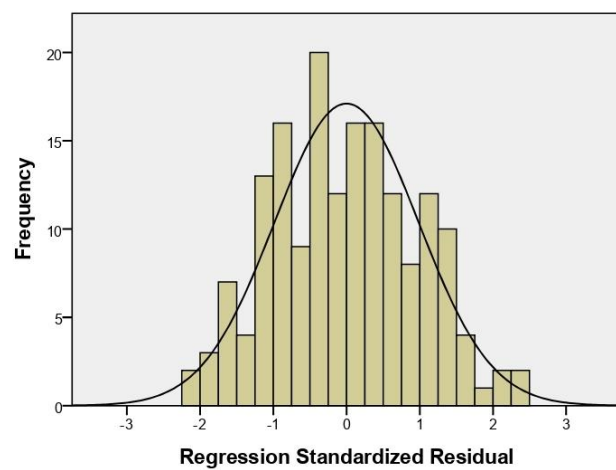
Supplementary Figure 1. Histogram of regression standardized residual for anxiety.
