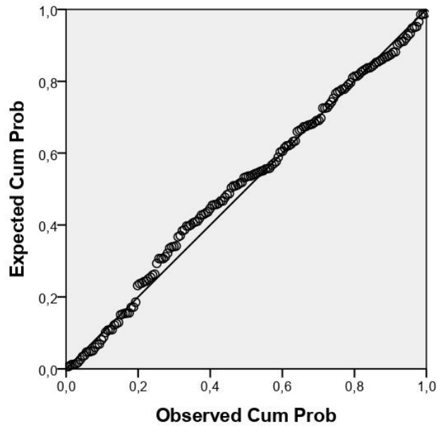
Supplementary Figure 7. Normal P-P plot of regression standardized residual for disability.
