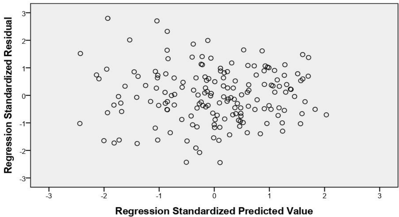
Supplementary Figure 12. Scatterplot of standardized residuals by standardized predicted values for psychological well-being.
