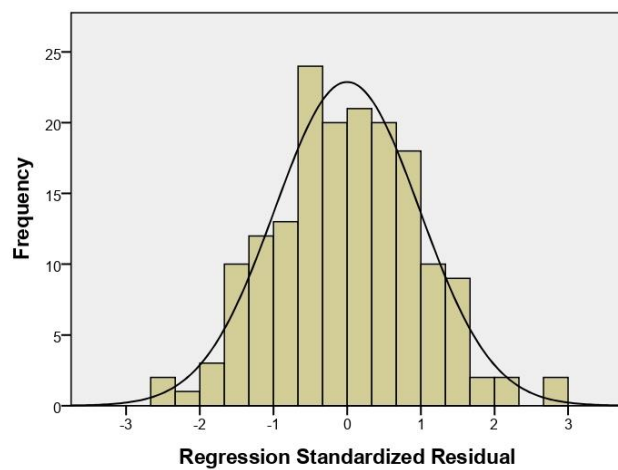
Supplementary Figure 2. Histogram of regression standardized residual for depression.
