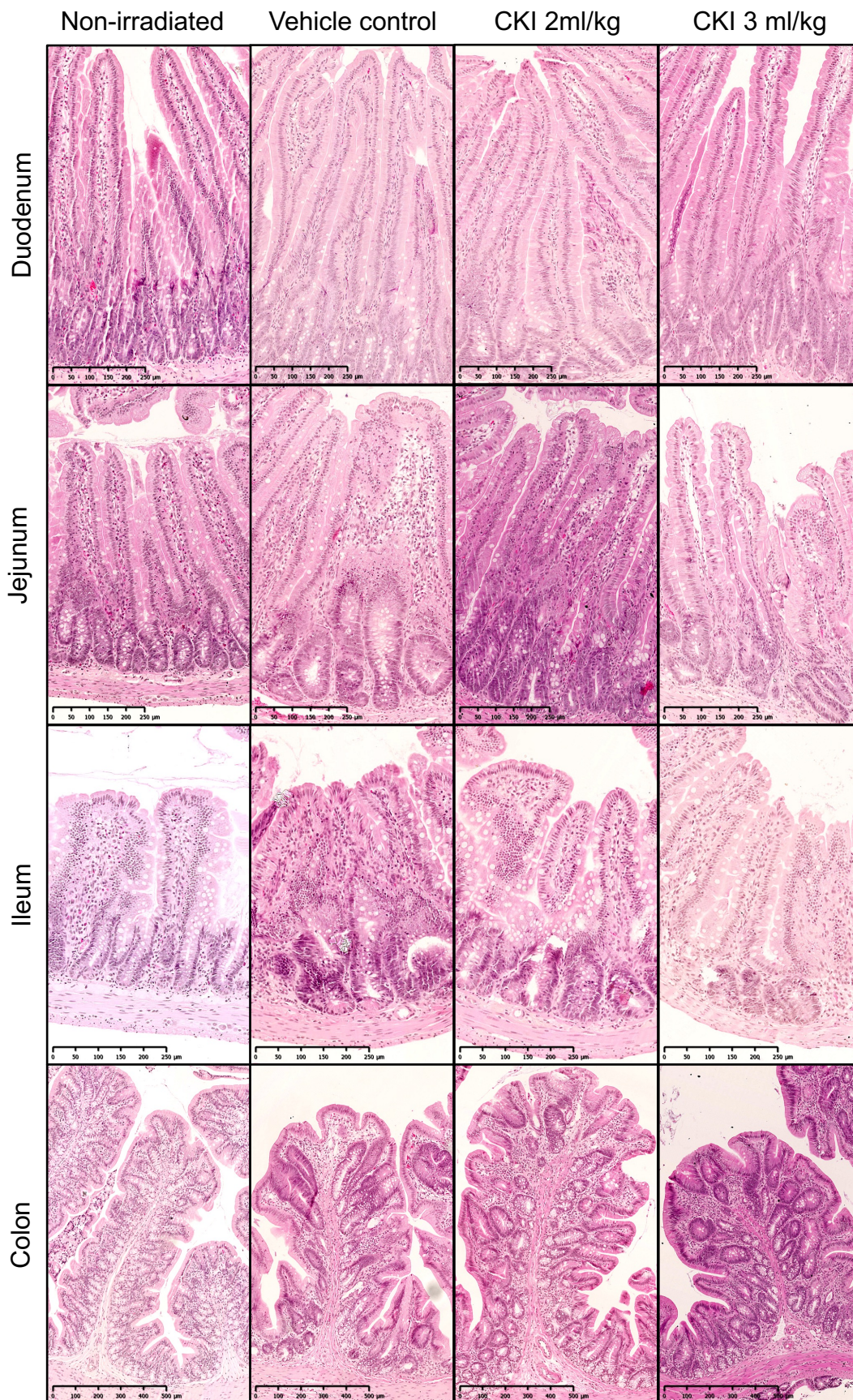
Supplementary figure 2: Administration of CKI reduces radiation induced mucosal damage. Representatives images of H and E stained duodenum and ileum sections from day 7 (a) and duodenum, jejunum, ileum and colon sections from day 11 (b). The intestines were collected from irradiated rats and paraffin-embedded tissues were sectioned for H & E staining.
