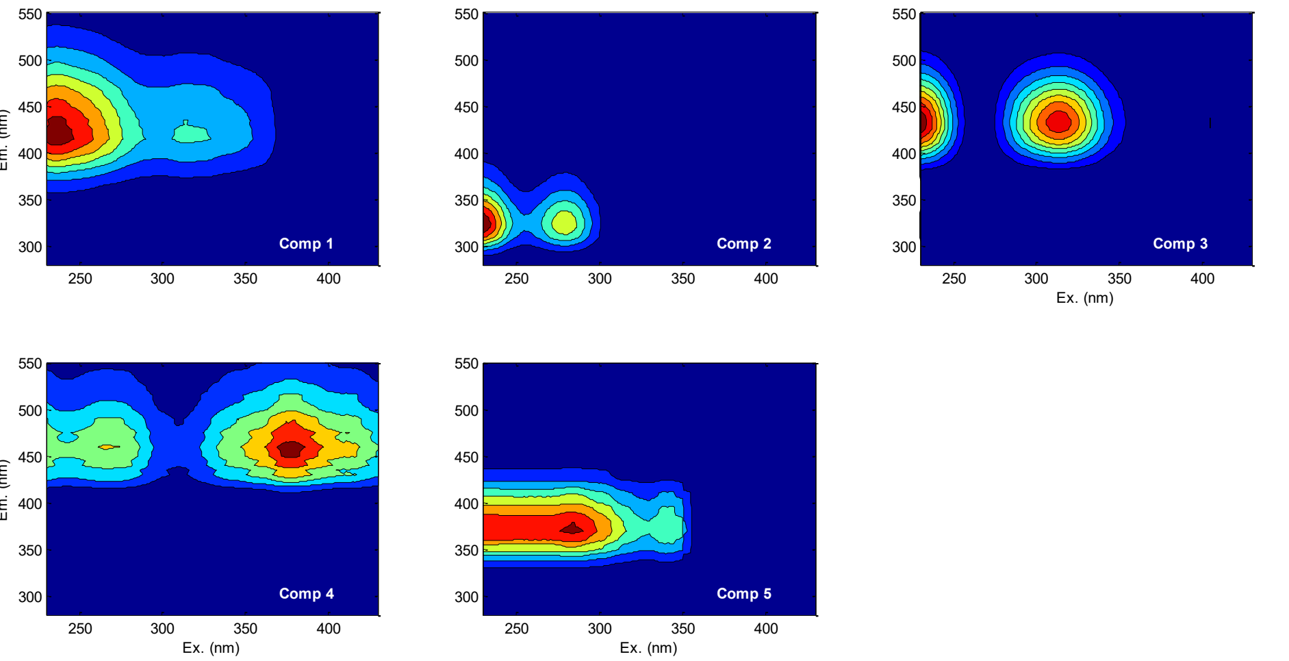
Figure S2- Component EEMs from PARAFAC model.
