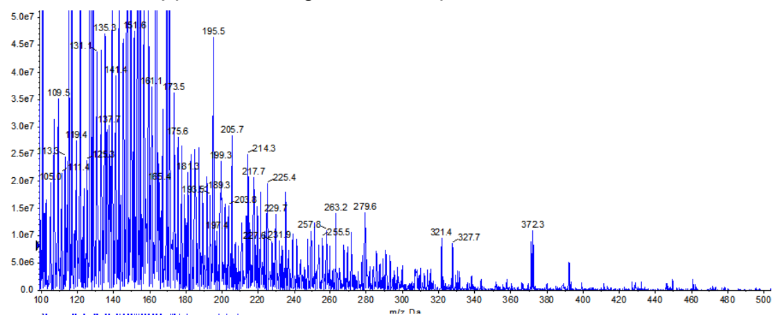
Figure S1- Raw mass spectra for balsam leachate that has been A) untreated, B) size-fractionated, and C) passed through the AF4 separation membrane.
