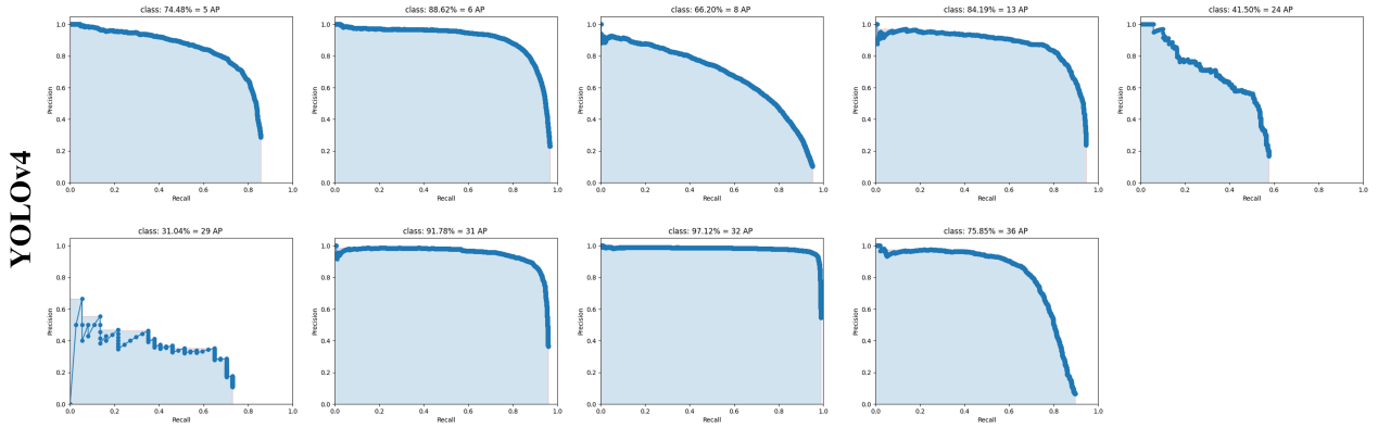
Figure S4. Precision-Recall graph showing the curves for YOLOv4 shown in Table 5.
