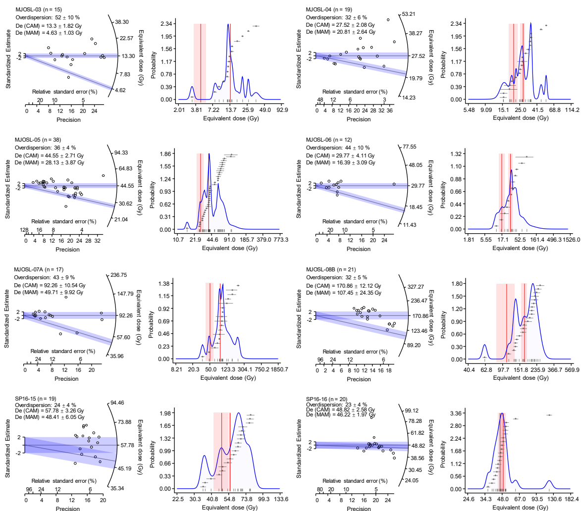
Figure, S1. Radial plots and probability density function (pdf) plots showing the De distributions. The two shaded areas refer to the 2σ range for the CAM and MAM De values.
