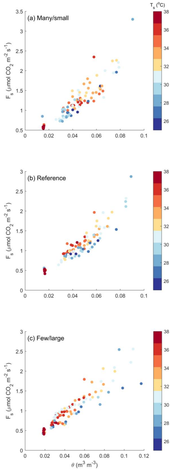
Supplementary Figure 3. Response of daily soil CO 2 efflux ( F_s ) to soil moisture ( \theta ) colored by soil temperature ( T_s ) for the three levels of rainfall repackaging.
