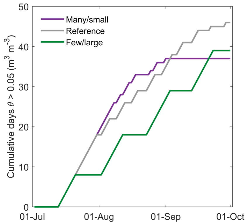
Supplementary Figure 1. Cumulative days with high soil moisture conditions (defined here as \theta exceeding 0.05 \text{ m}^3 \text{ m}^{-3} , the pooled mean of all daily \theta values, for the three levels of rainfall repackaging.
