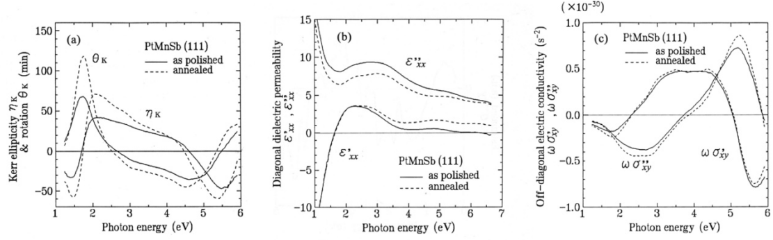
FIGURE S1 (a) Magneto-optical Kerr rotation and ellipticity spectra, and (b) spectra of real and imaginary parts and (c) spectra of real and imaginary parts of off-diagonal element of the dielectric permeability tensor in the as polished (solid line) and annealed (dotted line) {111} surfaces of a PtMnSb single crystal.
