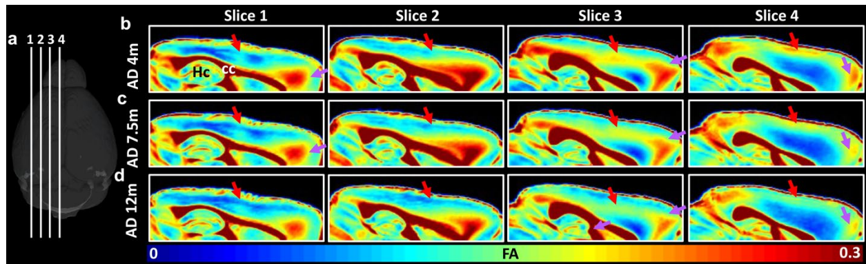
Supporting Information Figure S2. The representative slices showing the FA changes with age (4, 7.5, and 12 months) at cortex regions in 5xFAD mice.
